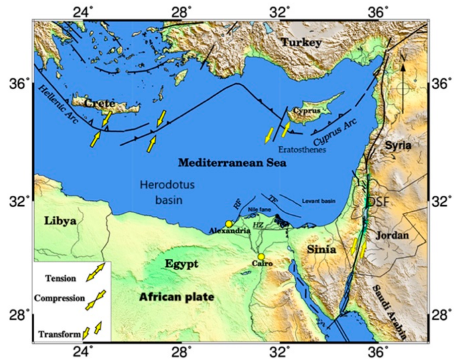
Figure 2. Main tectonic boundaries in the Eastern Mediterranean region, illustrating the Hellenic Arc, Cyprus Arc, Rosetta fault (RF), Tamsa fault (TF), and Hinge Zone fault which indicated by the black lines. The small yellow circles indicate the main cities. The yellow arrows indicate present-day stress in and around Egypt and are derived from Ali and Badreldin [31]. Detailed mapping of the fault is derived from [24,36].
