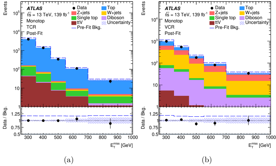
Figure 5. Comparison of data and SM prediction for the E_T^{\text{miss}} distribution in control regions targeting (a) t\bar{t} and (b) V +jets processes. The background predictions with the corresponding uncertainties result from the simultaneous fit to data in control and signal regions under the background-only hypothesis (Post-Fit). The signal regions included in the fit correspond to those targeting the scalar DM mediator production. The dashed line indicates the pre-fit total background prediction. The last bin of the distribution contains the overflow.
