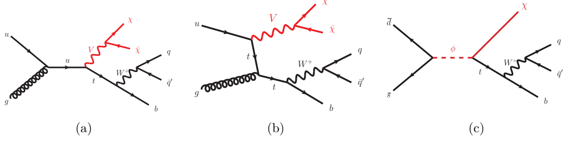
Figure 1. Representative Feynman diagrams for the DM production in association with a single top-quark decaying hadronically in the (a,b) vector mediator (non-resonant) and (c) scalar mediator (resonant) cases.
