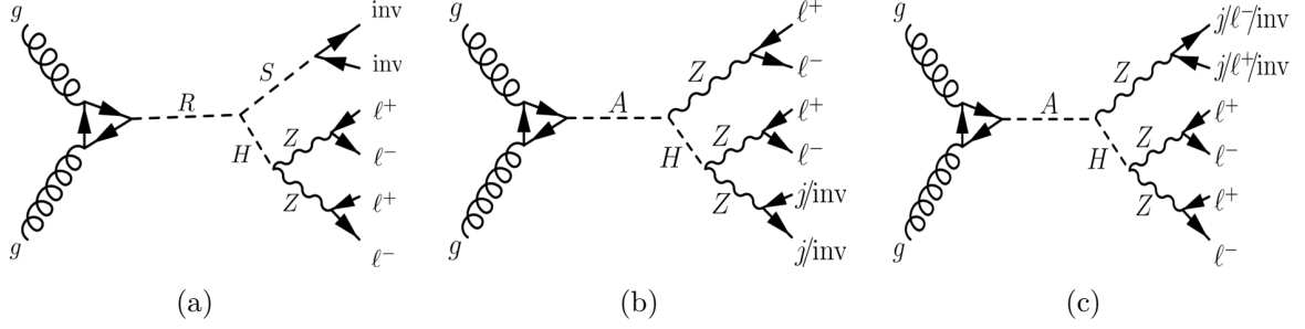
Figure 1. Feynman diagrams representing the production of heavy bosons via gluon-fusion at leading-order for the (a) R \rightarrow SH \rightarrow 4\ell + E_T^{\text{miss}} signal, (b) A \rightarrow Z(\rightarrow 2\ell)H(\rightarrow 2\ell + jj/\text{invisible}) signal, and (c) A \rightarrow Z(\rightarrow jj/\ell^+\ell^-/\text{invisible})H(\rightarrow 4\ell) signal, where \ell could either be an electron or a muon, j represents a jet and inv denotes an invisible particle.
