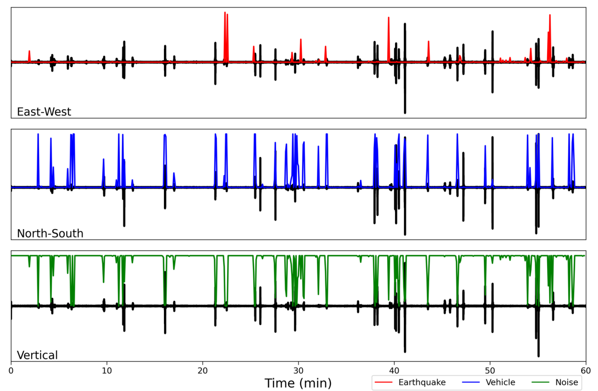
Fig. 6 Model prediction of noise, earthquake, and vehicle classes an hour-long seismic trace vehicle passing recorded at BEL7 station on 20th of January 2023 between 18:00 and 19:00 (UTC). Green, blue, and red lines with dots indicate model pre-
