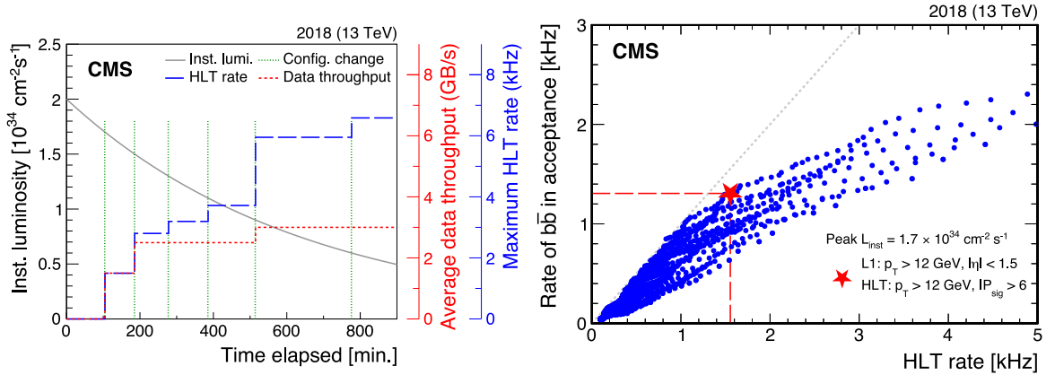
Fig. 39. Left: an example scenario in which the \mathcal{B} parking data throughput per L1 trigger setting is adjusted to maintain an average of approximately 2GB/s throughout an LHC fill. The dotted red and dashed blue lines trace the \mathcal{B} parking data throughput and maximum allowed HLT rate, respectively, determined for each trigger configuration. Changes in the trigger configuration are indicated by vertical green dashed lines. The trigger logic is adjusted to operate close to the permitted HLT rate. Right: rate of b\bar{b} events in acceptance versus HLT rate for a parameter scan over p_T and IP_{sig} thresholds imposed in the HLT logic for the \mathcal{L}_{inst} and L1 requirements indicated in the legend; each point (blue circle) represents a unique pair of thresholds and the red star indicates the optimal pairing of p_T > 12 GeV and IP_{sig} > 6 at a peak \mathcal{L}_{inst} = 1.7 \times 10^{34} \text{ cm}^{-2} \text{ s}^{-1} and an HLT rate close to the maximum allowed value of \approx 1.5 kHz.
