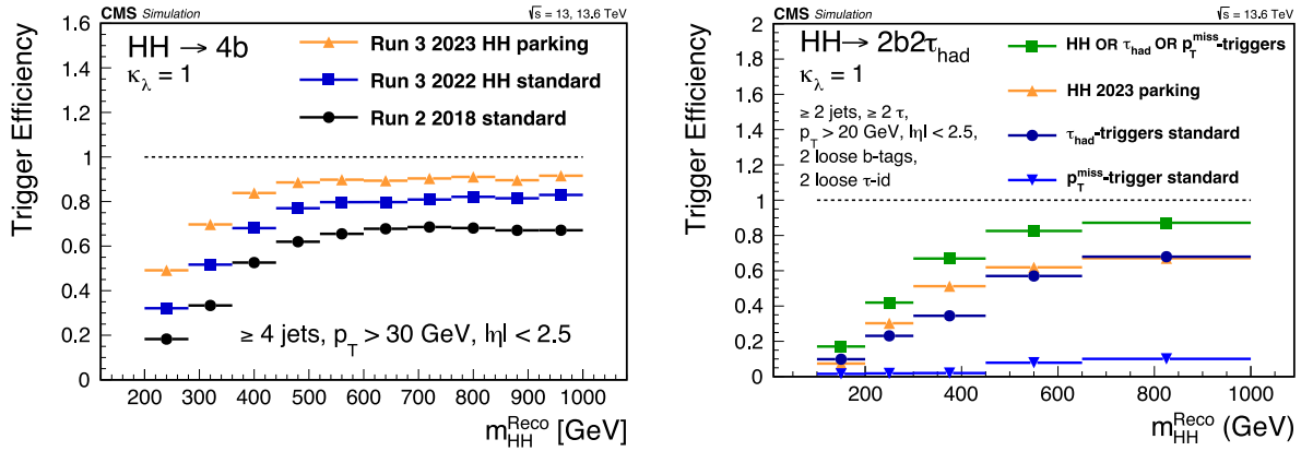
Fig. 60. Trigger efficiency for selecting signal HH events, plotted as a function of the reconstructed invariant mass of the two Higgs bosons, as measured in simulated HH → 4b (left) and HH → 2b2τ (right) samples corresponding to nominal Run 3 conditions.
