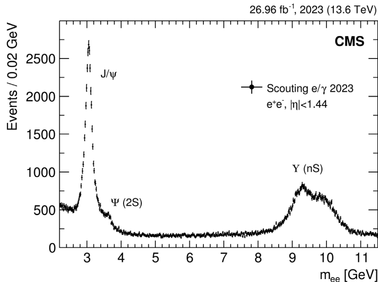
Fig. 37. Dielectron mass distribution observed with Run 3 scouting data collected during the 2023 data-taking period. The J/\psi and two of the \Upsilon meson peaks are visible.
