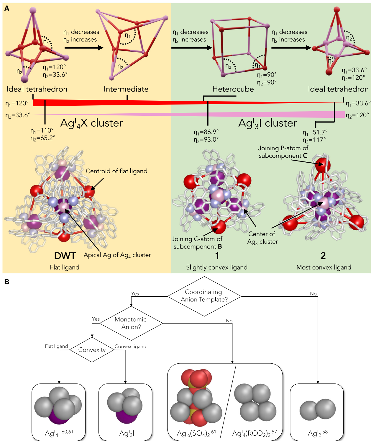
Figure 5. A taxonomy of silver-naphthyridine clusters that form cage vertices
