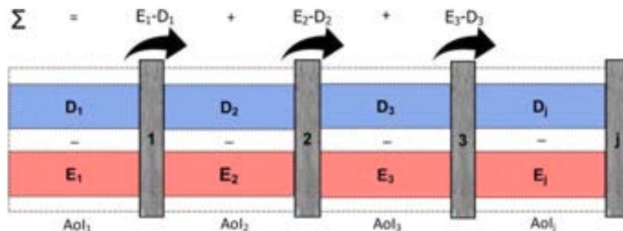
Fig. 3. Schematic representation of the SCR. For each Aol, the volume of sediment eroded (E), deposited (D) and the difference between the two, is involved. The cumulative net fraction of sediment passed over the upstream structures is also considered.
