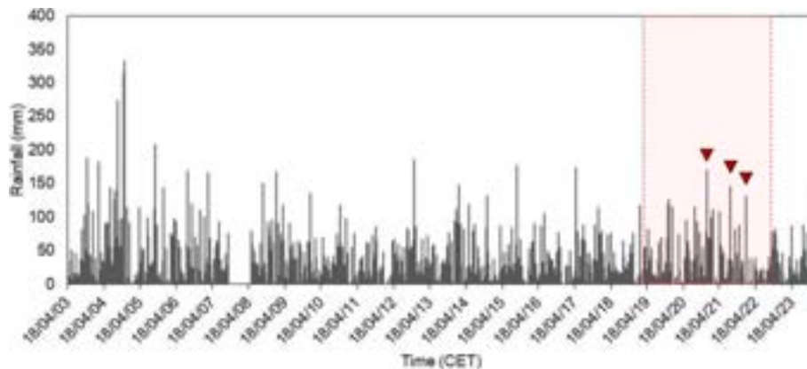
Fig. 4. Daily rainfall recorded by the Gemona del Friuli (307 m a.s.l.) meteorological station from April 2003 to October 2023. The red area refers to the 3-year study period, in which the three main rainfall events are identified.
