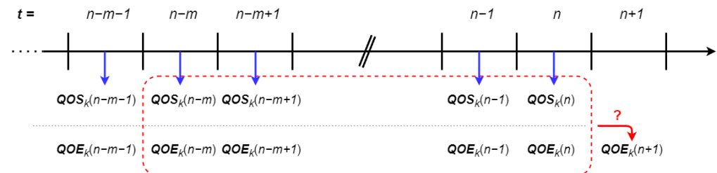
Figure 3. QoE prediction based on previous QoS/QoE samples.
