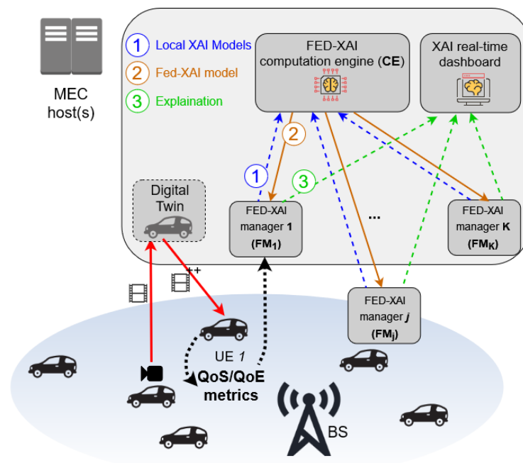
Figure 2. Example of video flow (red arrows) and related QoS/QoE metrics reporting (dashed black arrows) in a MEC-enabled FED-XAI architecture. Interaction among FM, CE and a real time XAI dashboard is also shown.
