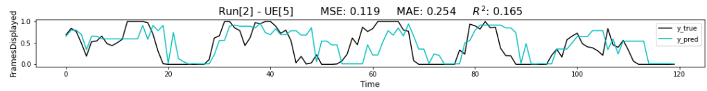
Figure 4. Real and predicted values of QoE for an example UE of the test set (Figure from [24]).
