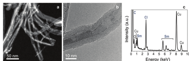
Fig. 1 (a) HAADF-STEM image of SmCl 3 @MWCNTs; (b) HRTEM image SmCl 3 @MWCNTs; (c) SmCl 3 @MWCNTs EDX spectrum showing the presence of samarium and chlorine atoms.
