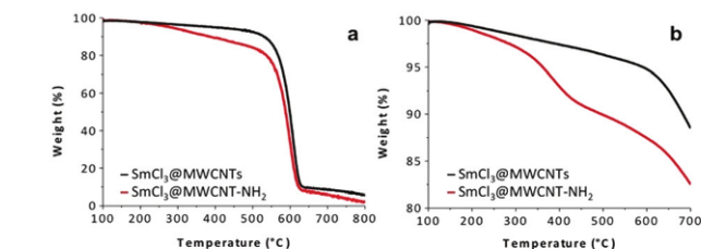
Fig. 2 TGA profiles of SmCl 3 @MWCNTs (—) and functionalized SmCl 3 @MWCNTs-NH 2 (—), (a) in air; (b) in N 2 atmosphere.
