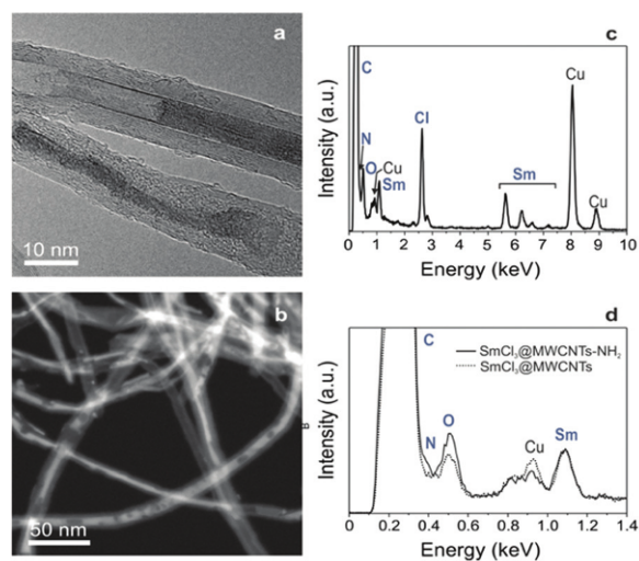
Fig. 3 (a) HRTEM image of SmCl 3 @MWCNTs-NH 2 ; (b) HAADF-STEM image of SmCl 3 @MWCNTs-NH 2 ; (c) EDX spectrum of SmCl 3 @MWCNTs-NH 2 ; (d) EDX spectra of SmCl 3 @MWCNTs-NH 2 (solid line) and SmCl 3 @MWCNTs (dotted line) in the 0–1.4 keV range.
