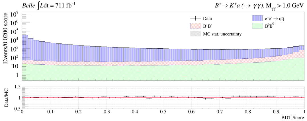
Figure 7. Distributions of the second continuum suppression BDT classifier scores. The colour convention used in this histogram is identical to that in figure 6.
