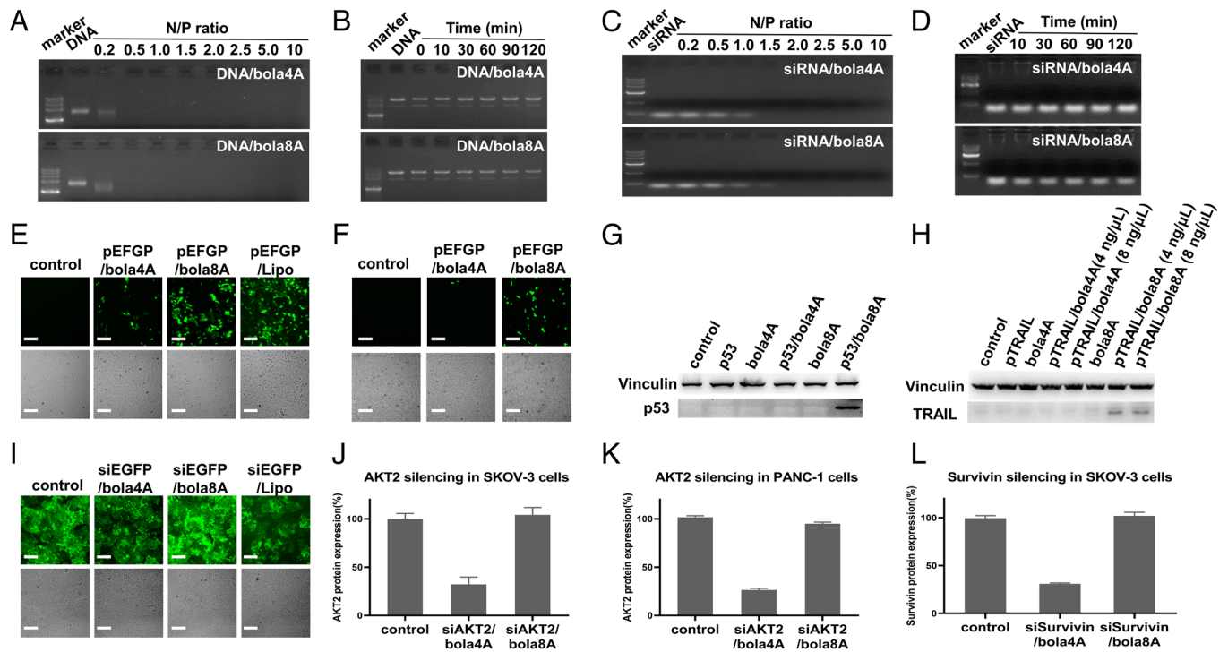
Fig. 2. Bola-amphiphilic dendrimers bola4A and bola8A bind both DNA and siRNA, but exert cargo-selective delivery. Agarose gel retardation assays of (A) DNA when binding with bola4A and bola8A at N/P ratios ranging from 0.2 to 10 (DNA 200 ng per well) and (B) DNA stability against DNase digestion in the presence of dendrimer at different time points (DNA 200 ng per well, N/P ratio of 1.0). Agarose gel retardation assays of (C) siRNA when binding with bola4A and bola8A at N/P ratios ranging from 0.2 to 10 (siRNA 200 ng per well) and (D) siRNA stability against RNase in the presence of dendrimer at different time points (siRNA 200 ng per well, N/P ratio of 10). DNA and siRNA delivery mediated by the bola-amphiphilic dendrimers bola4A and bola8A , respectively. GFP protein expression in (E) SKOV-3 cells and (F) HeLa cells following treatment with the DNA/dendrimer complexes using the pEGFP (12 and 4.0 ng/ \mu L DNA at N/P ratio of 1.0). Upper panel : fluorescent images; Lower panel : field images. Western blotting analysis of protein expression in HeLa cells upon treatment with the DNA/dendrimer complexes using (G) the plasmid DNA encoding the tumor suppressor protein p53 (p53) (12 ng/ \mu L DNA, N/P ratio of 1.0) and (H) the plasmid DNA encoding pTRAIL (4.0 and 8.0 ng/ \mu L DNA, N/P ratio of 1.0). (I) GFP expression after treatment of HeLa-GFP cells with siRNA/dendrimer complexes using the siRNA targeting GFP (siEGFP) (50 nM siRNA, N/P ratio of 10). Upper panel : fluorescent images; Lower panel : field images. Protein expression of protein kinase B (AKT2) in (J) SKOV-3 and (K) PANC-1 cells, and (L) Survivin in SKOV-3 cells after treatment with the siRNA/dendrimer complexes using the siRNAs targeting AKT2 (siAKT2) and Survivin (siSurvivin) respectively (50 nM siRNA, N/P ratio of 10). The commercial transfection reagent Lipo2000 (Lipo) was used as a control. pEGFP: plasmid DNA expressing GFP; p53: plasmid DNA expressing tumor suppressor protein p53; pTRAIL: plasmid DNA expressing TRAIL; siEGFP: siRNA targeting GFP; siAKT2: siRNA targeting AKT2; siSurvivin: siRNA targeting Survivin. *** P < 0.001 (mean \pm SD, n = 3 ).
