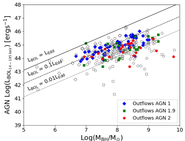
Figure 5. Bolometric luminosity as a function of SMBH mass for our sample. Symbols are identical to Fig. 4. The lines correspond to L_{\text{Bol}} = L_{\text{Edd}} (solid), L_{\text{Bol}} = 0.1 L_{\text{Edd}} (dashed), and L_{\text{Bol}} = 0.01 L_{\text{Edd}} (dotted).
