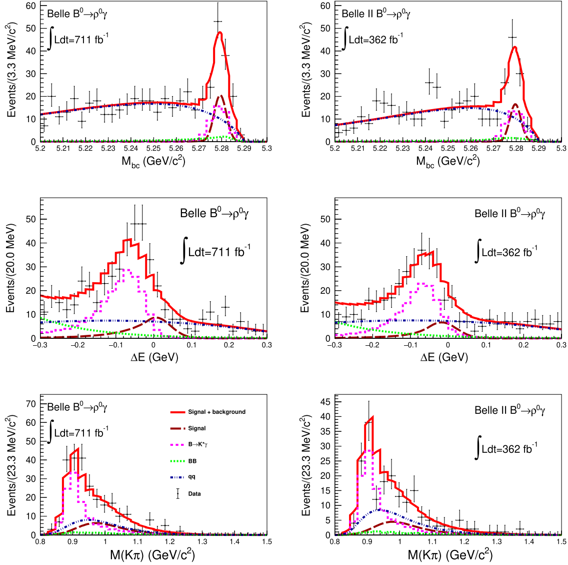
FIG. 4. Distributions of M_{bc} , \Delta E and M(K\pi) for B^0 \rightarrow \rho^0 \gamma candidates reconstructed in the signal-enriched region of the other two variables. The signal-enriched region is defined as M_{bc} > 5.27 \text{ GeV}/c^2 , |\Delta E| < 0.1 \text{ GeV} and M(K\pi) > 0.92 \text{ GeV}/c^2 . The points with error bars are data, the solid red curves are the sum of signal and background PDFs, the dashed red curves are signal, the dotted-dashed blue curves are continuum background, the dashed magenta curves are K^* \gamma background, and the dotted green curves are B\bar{B} background other than K^* \gamma . The discrete nature of the solid red curves, which represent the signal + background fit, is due to the use of histogram PDFs for some of the backgrounds, as described in the text.
