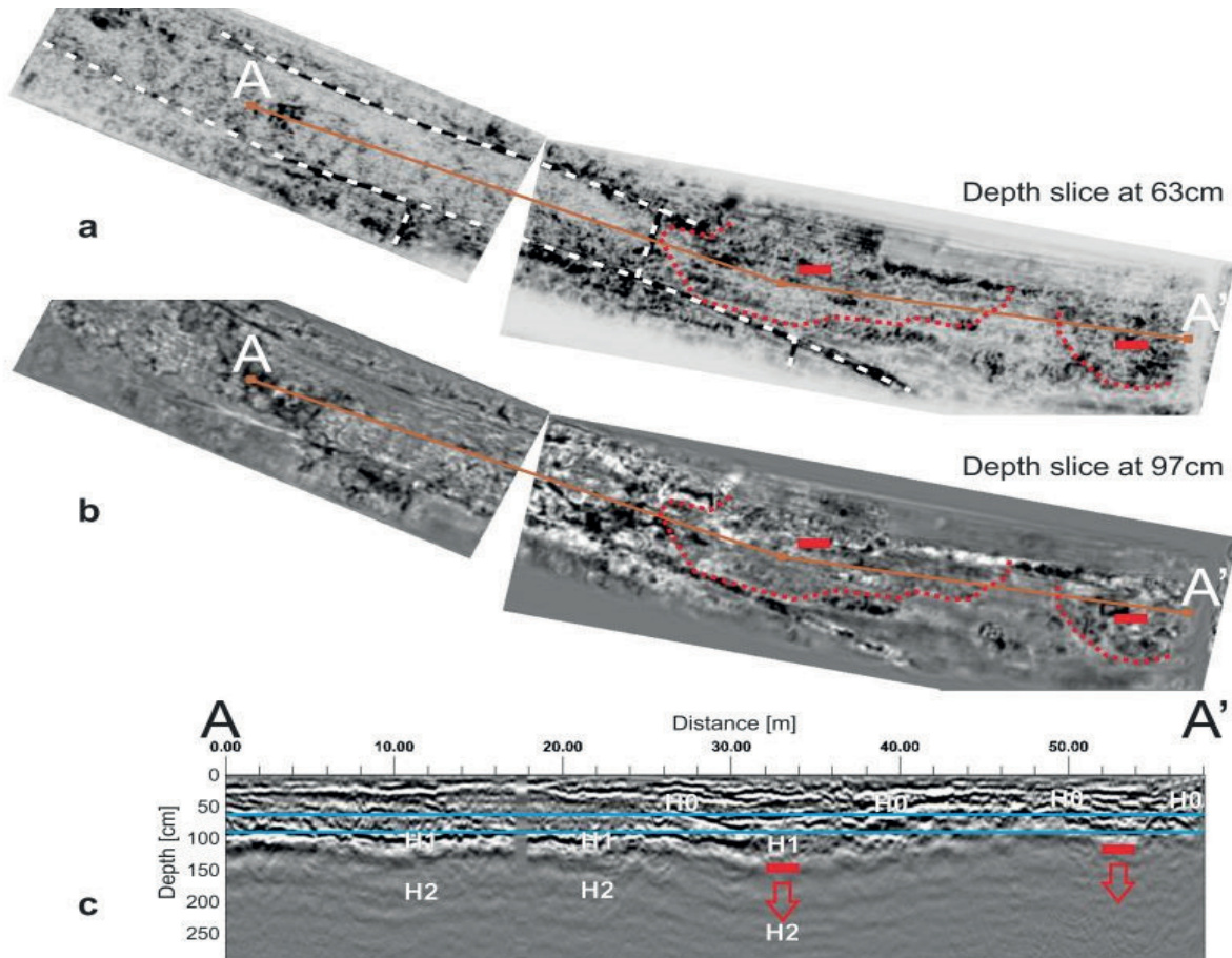
Fig. 3 - Example of results of full 3D GPR surveys. a) and b) are two exemplary depth slices at 63 and 97 cm below the topographic surface, respectively, while in c) a profile crossing the area is shown. All red features are related to two interpreted depocenters: dotted lines mark their lateral extension, while the arrows the maximum deformation. Dashed white lines highlight some of the various pipes present in the area. Blue lines in c) mark the depth of the two depth slices in a) and b). H0, H1, H2 are GPR horizons, see text for further details
