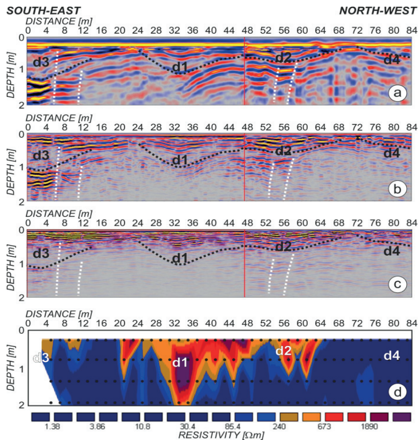
Fig. 2 - Processed and interpreted GPR profiles acquired with different antennas: a) 250 MHz; b) 500 MHz; c) 800 MHz, compared with an ERT (d) acquired along the same path (inverted data). d1, d2, d3 and d4 highlight the positions of 4 depocenters marked by black dotted lines. White dotted lines mark the main lateral variations. Red vertical segments on the GPR profiles depict the transition between two different road pavements (modified after ZINI et alii, 2015)
