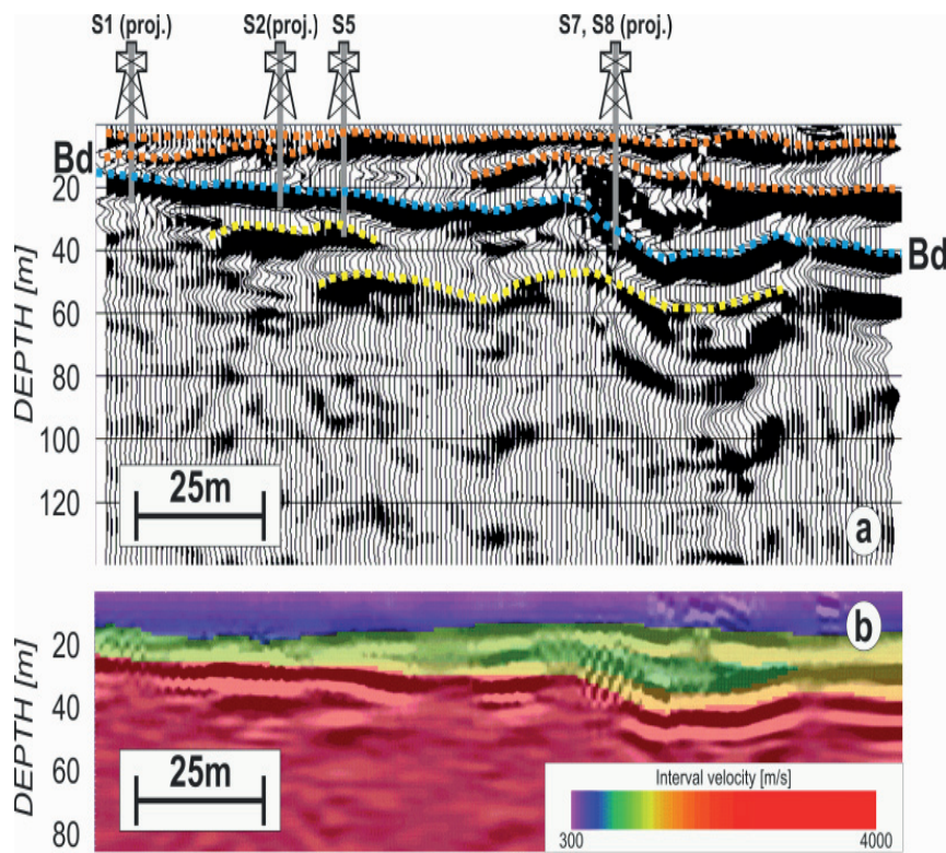
Fig. 4 - Exemplary reflection seismic section (modified after BUSETTI et alii, 2020). a) Processed and interpreted section; b) seismic interval velocity field (P-waves) superimposed on the seismic section as in a). The evaporitic bedrock (Bd) is clearly imaged and shows a strong velocity increment up to values typical of evaporites. Other horizons can be recognized both above (in orange) and within (in yellow) the bedrock. Some boreholes validate the seismic results
