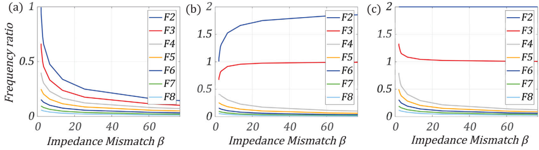
Fig. 5. Plots of functions (a) f_i^{1st}/f_c , (b) f_i^{2nd}/f_c and (c) \tilde{f}_i/f_c as a function of impedance mismatch \beta (canonical ratio C = 1 ).
