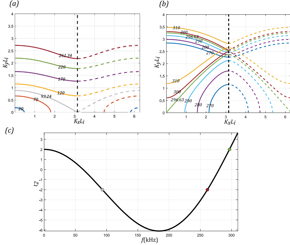
Fig. 2. Laminate F_2 combining PMMA and steel. (a), (b) Plots of real solutions of the dispersion equation in the graph K_y L_i vs K_x L_i for several given frequencies; in particular, (a) f \in [20, 261.34] kHz, for each selected frequency and selected K_x L_i , either none or one mode of propagation is displayed, (b) f \in [270, 296.63] kHz, for each selected frequency and selected K_x L_i , either one or two modes of propagation are displayed. (c) Plot of trace t_2(f, 0) , the grey point marks the upper limit of the first pass band, the red one that of the first stop band and the green one that of the second pass band.
