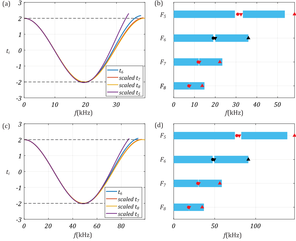
Fig. 4. Scaling of traces at low frequencies in the vicinity of f = 0 . Plot of traces for (a) C = 1/5 , \beta = 13.520 and (c) C = 1 , \beta = 3.351 ; in both plots, the adopted scaling factor is \phi . (b), (d) Plot of the first two pass bands with prediction of their limits (indicated by red markers) obtained using the scaling factor \phi starting from the exact limits of the pass bands for F_6 (black markers).
