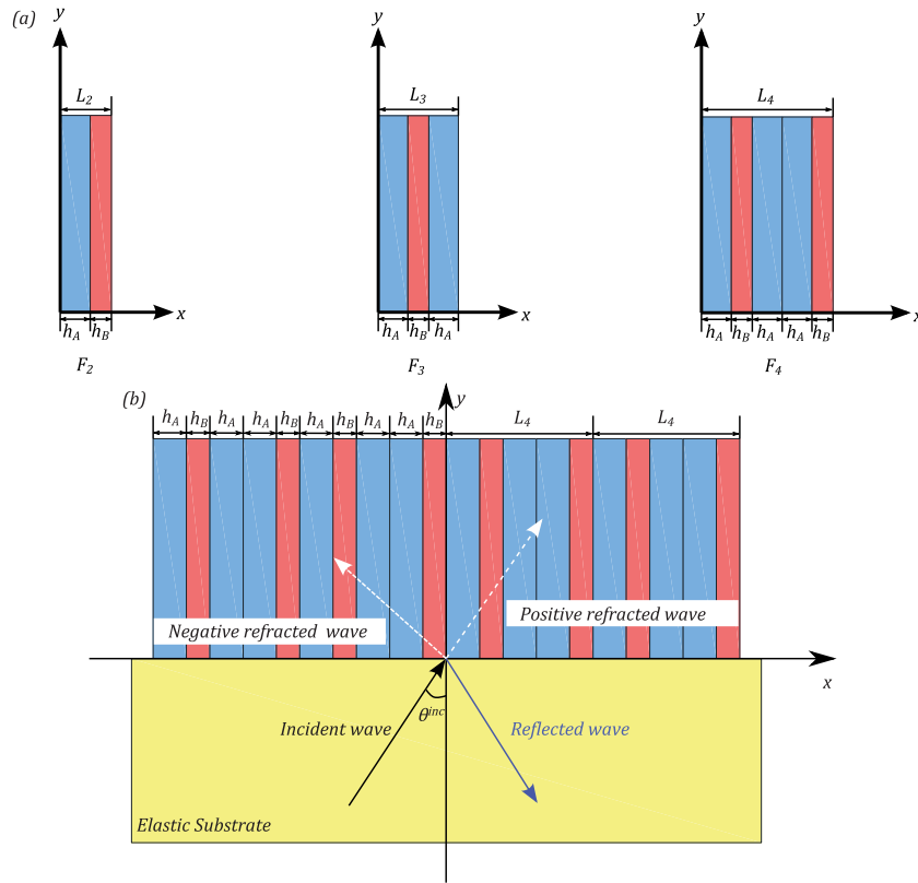
Fig. 1. (a) Elementary cells for Fibonacci sequences F_2 , F_3 and F_4 ; (b) reflection and refraction of an anti-plane shear wave approaching the interface between an elastic substrate and a Fibonacci laminate F_4 .
