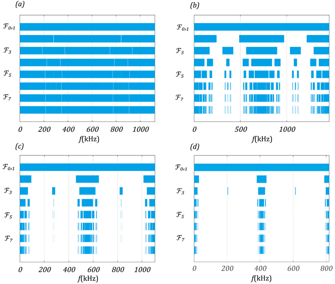
Fig. 3. Stop- and pass-band layout (pass bands in light blue) for canonical Fibonacci laminates with four different impedance mismatches, but same canonical ratio C^{(1)} = 1 . (a) Material A : iron, material B : copper, \beta = 2.0002 ; (b) A : steel, B : aluminium, \beta = 3.351 ; (c) A : PMMA, B : steel, \beta = 13.520 ; (d) A : steel, B : polyethylene, \beta = 76.706 . In each plot, sequences \mathcal{F}_0 to \mathcal{F}_8 are displayed and the maximum value of the frequency is 4f_c .
