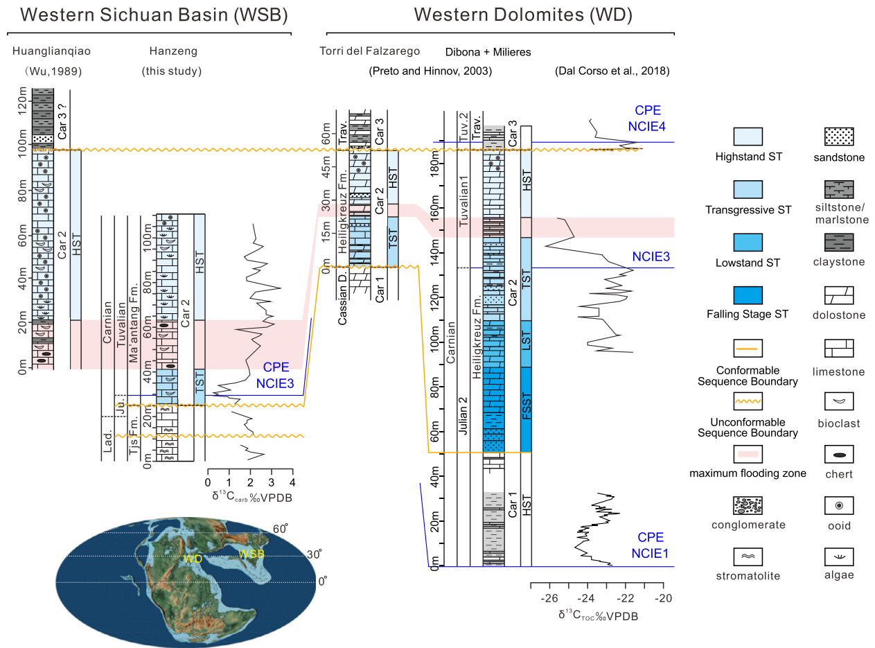
Fig. 4. Bio- chemo- and sequence stratigraphic correlation of the Hanzeng section (31°47′06″N; 104°37′48″E) in the Sichuan Basin with coeval sections of Torri del Falzarego (46°31′40″N; 12°1′18″E) and Dibona+Milières (46°32′2″N; 12°4′20″E) in the Western Dolomites. The organic carbon isotope records from the marine successions of the Western Tethys are taken from Dal Corso et al. (2018). Lad. = Ladinian; Ju. = Julian; Tuv. = Tuvallian; Tjs = Tianjingshan Fm.; Trav. = Travenanzes Fm.; Lag. = Lagazuoi Member. Paleogeographic map of Carnian (Late Triassic) is based on Scotese (2014).
