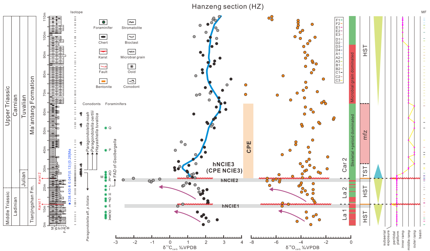
Fig. 2. Microfacies, \delta^{13}\text{C} , \delta^{18}\text{O} , and bio-chronostratigraphy of the Hanzheng section. Three negative carbon isotopic excursions (hNCIE1 to 3) are identified. The descriptions of the microfacies (MF) F1 to C3 are shown in the Supplemental Dataset. M = Mudstone; W = Wackestone; P = Packstone; G = Grainstone; F = Floatstone; B = Boundstone; HST = Highstand System Tract; LST = Lowstand System Tract; Mfz = Maximum flooding zone; CPE = Carnian Pluvial Episode; FAD = First Appearance Datum. In the \delta^{13}\text{C} data, black dots refer to samples whose \delta^{18}\text{O} values are within the range of articulate brachiopod \delta^{18}\text{O} values reported by Korte et al. (2005) and are therefore considered little affected by diagenesis. Gray dots are instead samples that are thought to be altered because of diagenetic phenomena. Blue line is locally weighted scatterplot smoothing (LOWESS) of non-diagenetic \delta^{13}\text{C} values above Karst 2. The NCIE1 and NCIE2 of the CPE are not preserved in this section.
