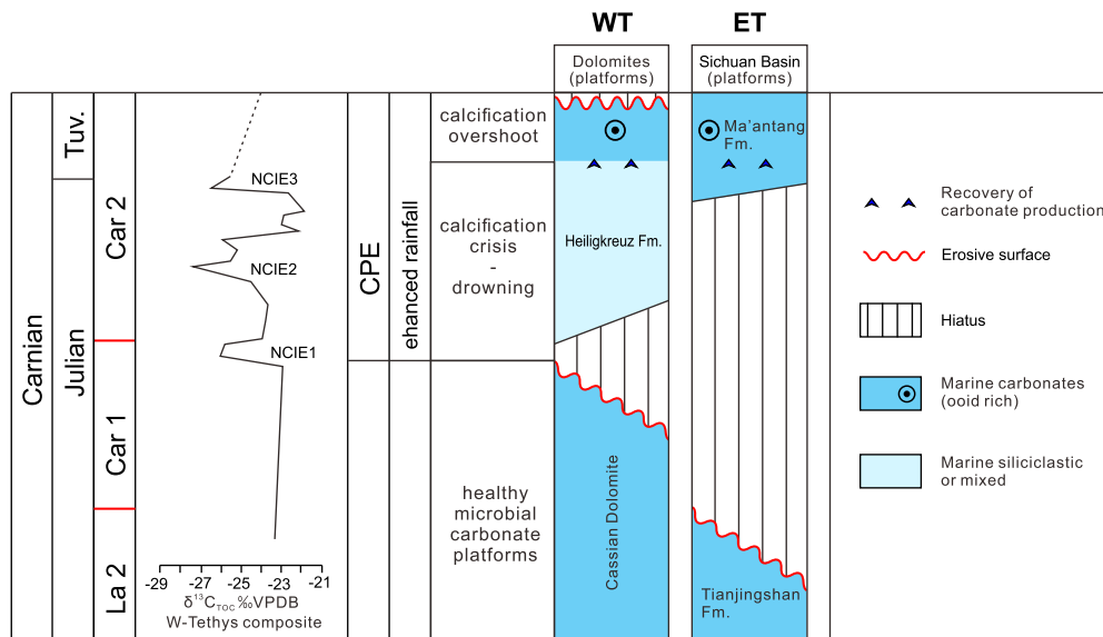
Fig. 5. Schematic representation of how carbonate production might have evolved in shallow water marine environments during the transgressive part of the CAR2 sequence. The \delta^{13}\text{C}_{\text{TROC}} curve is a composite from Dal Corso et al. (2018). The hypothesized calcification overshoot within the CAR 2 sequence precedes the recovery of microbial carbonate production that has been observed after the CPE and that did not happen prior the end of the Tuvanian (Jin et al., 2020). WT = western Tethys; ET = eastern Tethys.
