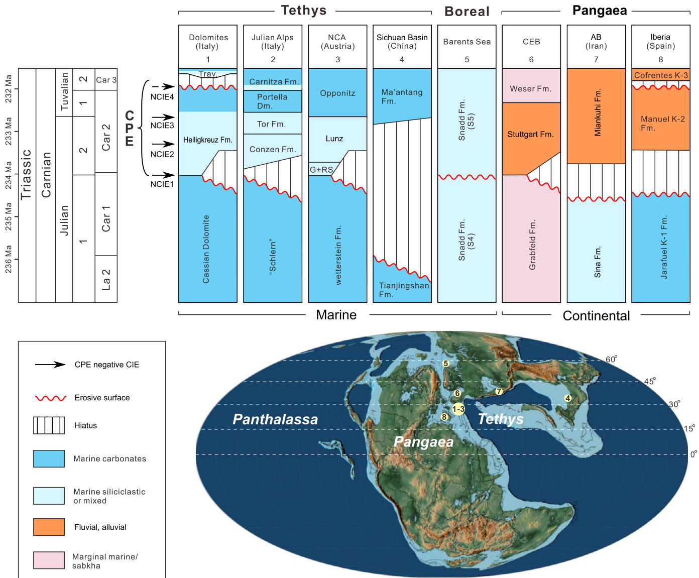
Fig. 3. Record of the Julian eustatic sea-level fall in the marine (Tethyan and Boreal) and continental realms (Pangaea). 1. Dolomites (Dal Corso et al., 2018, and references therein); 2. Julian Alps (Dal Corso et al., 2018, and references therein); 3. Northern Calcareous Alps (Mueller et al., 2016); 4. Sichuan Basin (this work); 5. Barents Sea (Klausen et al., 2020); 6. Central European Basin (CEB, Franz et al., 2014; Zhang et al., 2020); 7. Aghdarband Basin (AB, Northeast Iran, Mazaheri-Johari et al., 2022); 8. Iberia and Balearic Islands (Barrenechea et al., 2018; Ortí et al., 2017). G+RS = Göstling Mb. and Reingraben Shales. Paleogeographic location of the succession is shown on map of Carnian (Late Triassic) from Scotese (2014).
