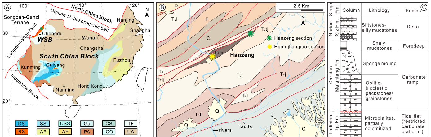
Fig. 1. A) The Carnian palaeogeographical map of South China (modified from Ma et al., 2009). The green marker represents the location of the Hanzeng section. WSB: Western Sichuan Basin; DS: deep sea; SS: shallow sea; CSS: coast to shallow sea; GU: gulf; CS: coastal swamp; TF: tidal flat; RS: reef mound and shoal; AP: alluvial plain; AF: alluvial fan; PA: paleoland; CO: coast; UA: uplift area. B) Geological map (modified from 1:50000 Geological Map of the Jiangyou Map Sheet published in regional geological survey report, 1996) showing the location of the Hanzeng (green marker) and Huanglianqiao (yellow marker) sections in the Hanzeng area. D: Devonian; C: Carboniferous; P: Permian; J: Jurassic; T 1f : Feixianguan Fm., Lower Triassic; T 1j : Jialinjiang Fm., Lower Triassic; T 2l : Leikoupo Fm., Middle Triassic; T 2tj : Tianjingshan Fm., Middle Triassic; T 3m : Ma'antang Fm., Upper Triassic; Q: Quaternary. C) Lithological column and typical facies of Ladinian-Carnian (Tianjingshan Fm.), Carnian (Ma'antang Fm.) and early Norian (XTZ, Xiaotangzi Fm., modified from Jin et al., 2019). The red wavy line represents the flexural forebulge unconformity follows Jin et al. (2019). (For interpretation of the colors in the figure(s), the reader is referred to the web version of this article.)
