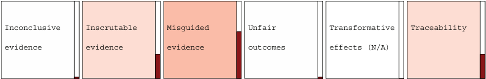
Fig. 5. Ethical challenge risk labels of the Communities and Crime dataset. Since the records of this dataset refer to communities and not individuals, we decided to exclude the DB measurement. The labels are calculated considering only DQ and DD.
