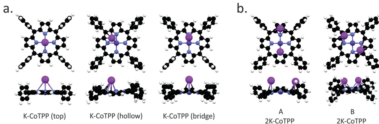
Fig. 6 A schematic representation of the different K adsorption geometries calculated for the K-CoTPP (a) and 2K-CoTPP (b) complexes. Black, white, light blue, and violet spheres represent C, H, N, Co, and K, respectively.
