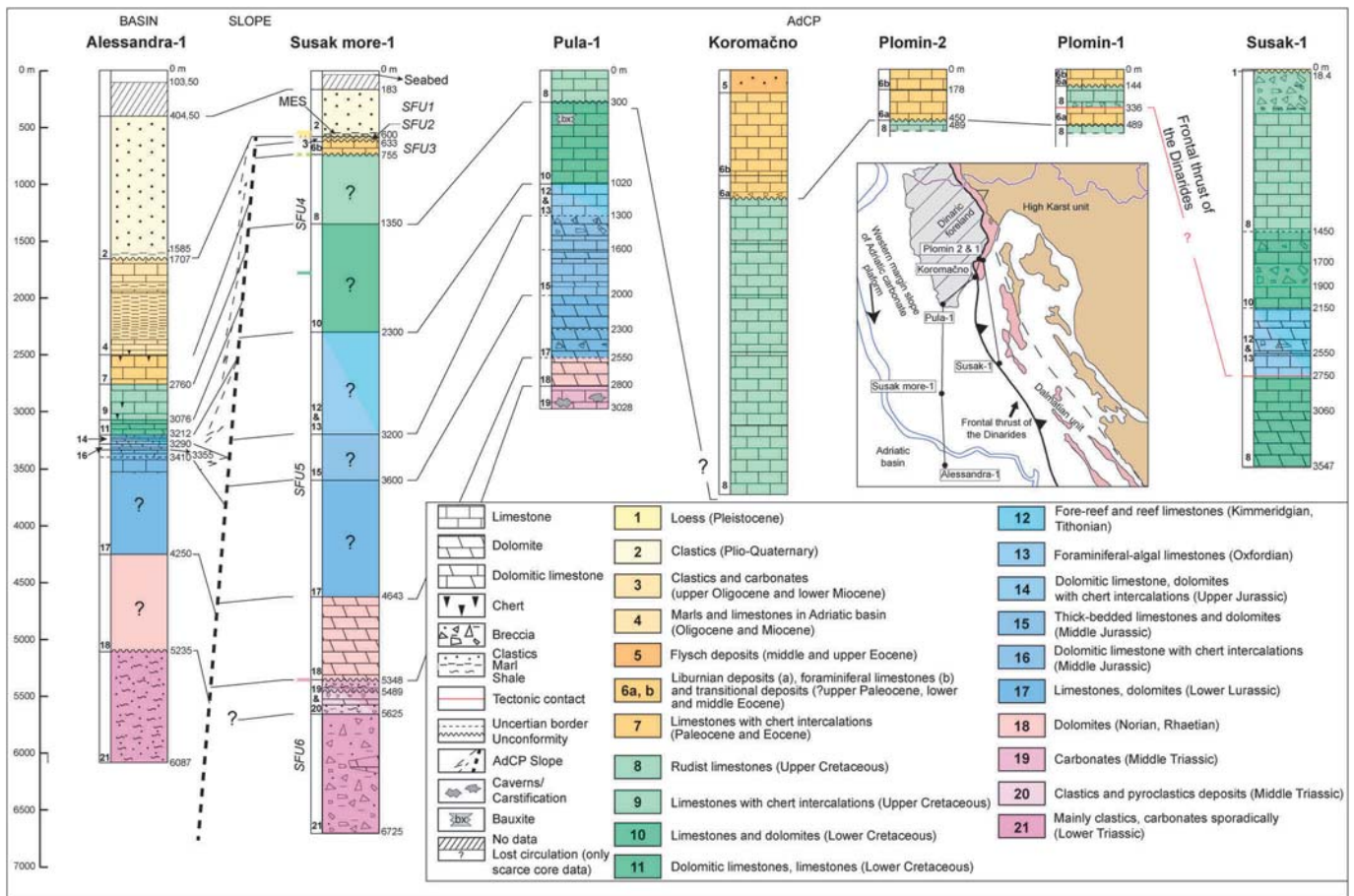
Fig. 3. Position (inset) and stratigraphic correlation of wells available in the study area (after Magaš, 1965; Grandić et al., 1999, Grandić et al., 2013; Velić et al., 2015; Schmid et al., 2020).
