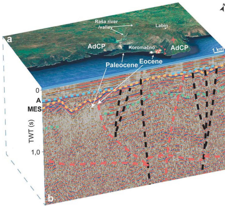
Fig. 10. Surface (a) to subsurface (b) correlation of major structures in the Koromačno-Labin outcrop area (position in Fig. 1): the structure continues in the western Cres Anticline.
