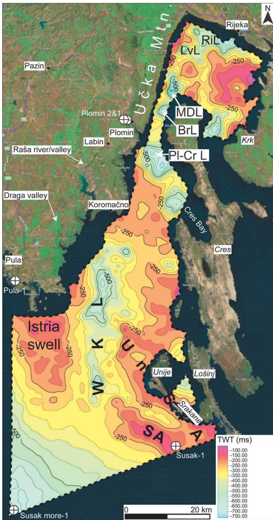
Fig. 13. Time structural map of the Messinian erosional surface. SA: Susak Anticline, WKL: West Kvarner lineament, PI-Cr L: Plomin-Cres Bay lineament, BrL: Brcelj low, MDL: Mošćenička Draga low, LvL: Lovran low, RiL: Rijeka low.
