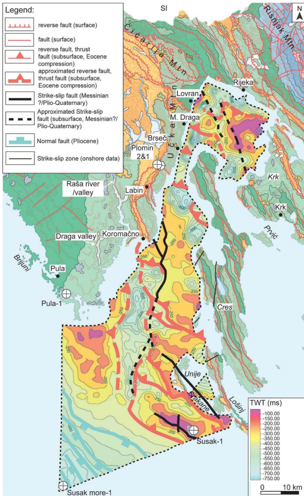
Fig. 16. An attempted correlation between onshore and offshore main faults on the MES structural map in the Kvarner area (onshore data from GKRH, 2009; Fuček et al., 2012; Fuček et al., 2015). Red lines are pre-MES thrust faults, black lines are Pliocene–early Pleistocene transpressive systems, often reactivating the previous thrust. (For interpretation of the references to colour in this figure legend, the reader is referred to the Web version of this article.)
