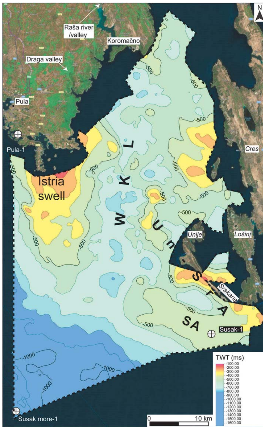
Fig. 12. Time structural map of the Barremian horizon, within the Lower Cretaceous carbonates. SA: Susak Anticline, WKL: West Kvarner lineament, Un-SrA: Unije-Srakane anticline.
