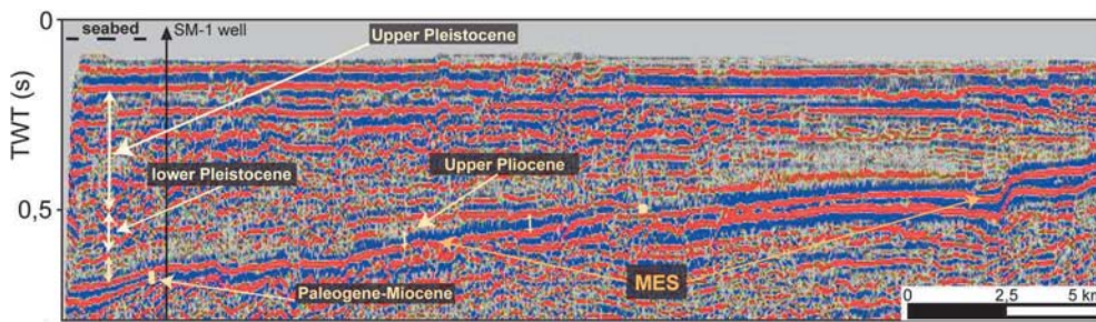
Fig. 5. Detail of the composite profile of Fig. 4: calibration by Susak more-1 well evidences the high amplitude Cenozoic packages; their thicknesses are at the limit of vertical seismic resolution. Note top lap termination of the Miocene-Paleogene layers on the left part of the profile. Vertical exaggeration is x10. See position in Fig. 2.
