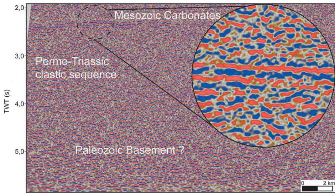
Fig. 7. Deep detail of the seismic profile sited in the western sector of the study area. High amplitude low-frequency reflectors typically characterize the seismic facies of the Permo-Triassic clastic sequence and allow to distinguish them from the upper carbonate succession.
