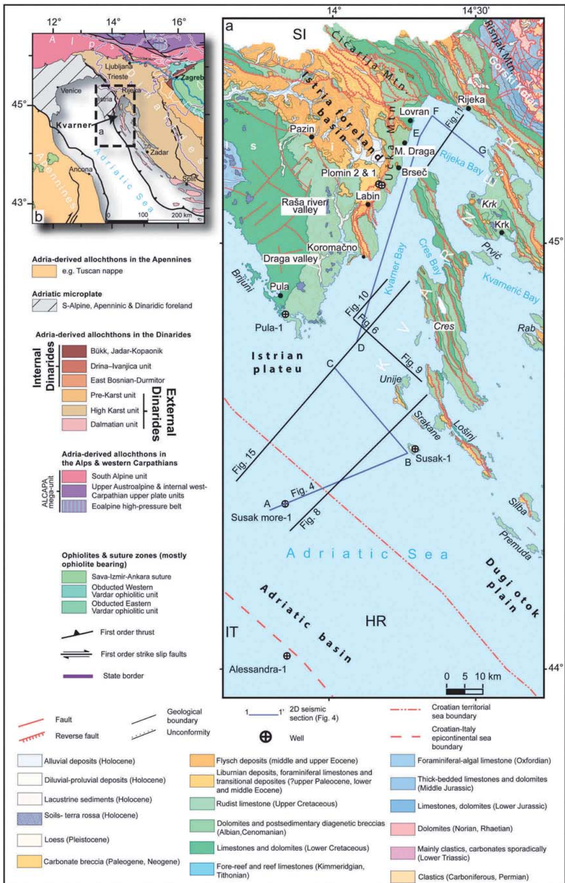
Fig. 1. Local geological (a) and regional geotectonic setting (b) of the study area (after Schmid et al., 2020; GKRH, 2009; https://www.azu.hr/en ).
