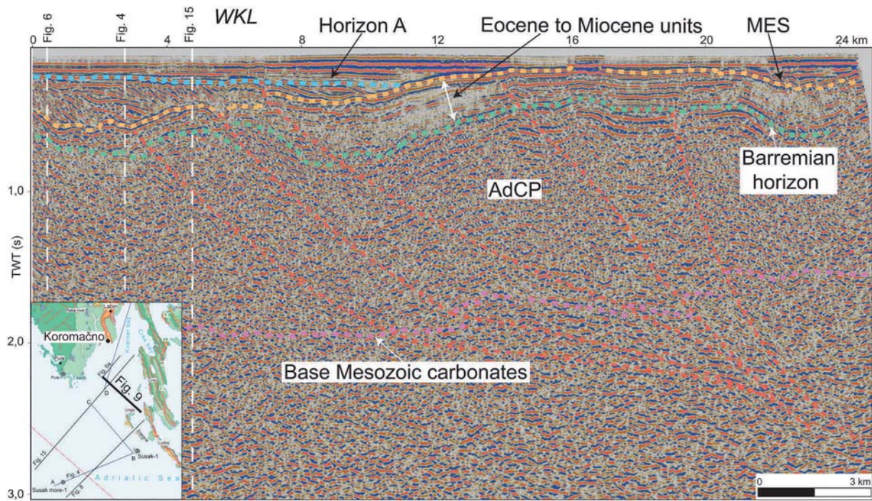
Fig. 9. Seismic profile crossing the W-Kvarner lineament. On the left, a clinoform system fills the channel downlapping to the MES. On the right, an Eocene thickness was interpreted, referred to as turbidite deposits of the Dinaric foreland. Thick-skinned tectonics was evaluated.
