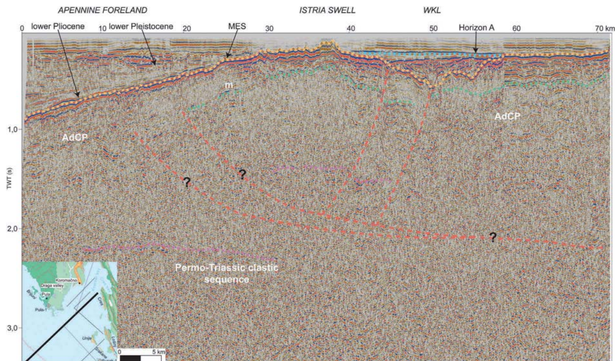
Fig. 15. Seismic profile crossing the southern offshore Istria Swell, here interpreted as related to compressive tectonics. The western side is emphasized by the westward tilting of the Apennine foreland.
