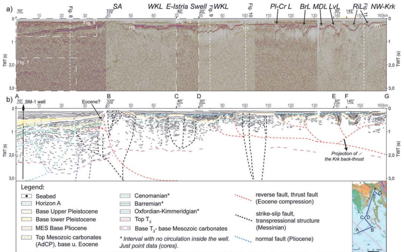
Fig. 4. Regional composite seismic section from the Adriatic Sea axis to the Rijeka coast, crossing the entire Kvarner area, between the SE-Istrian coast and the Lošinj/Cres/Krk Islands. (a) Uninterpreted profile and (b) line-drawing. Boxes in (a) are the details represented in the following pointed figures. SA: Susak Anticline, WKL: West Kvarner lineament, PI-Cr L: Plomin-Cres Bay lineament, BrL: Brseć low, MDL: Mošćenička Draga low, LvL: Lovran low, RiL: Rijeka low, SM: Susak more-1, m: multiples.
