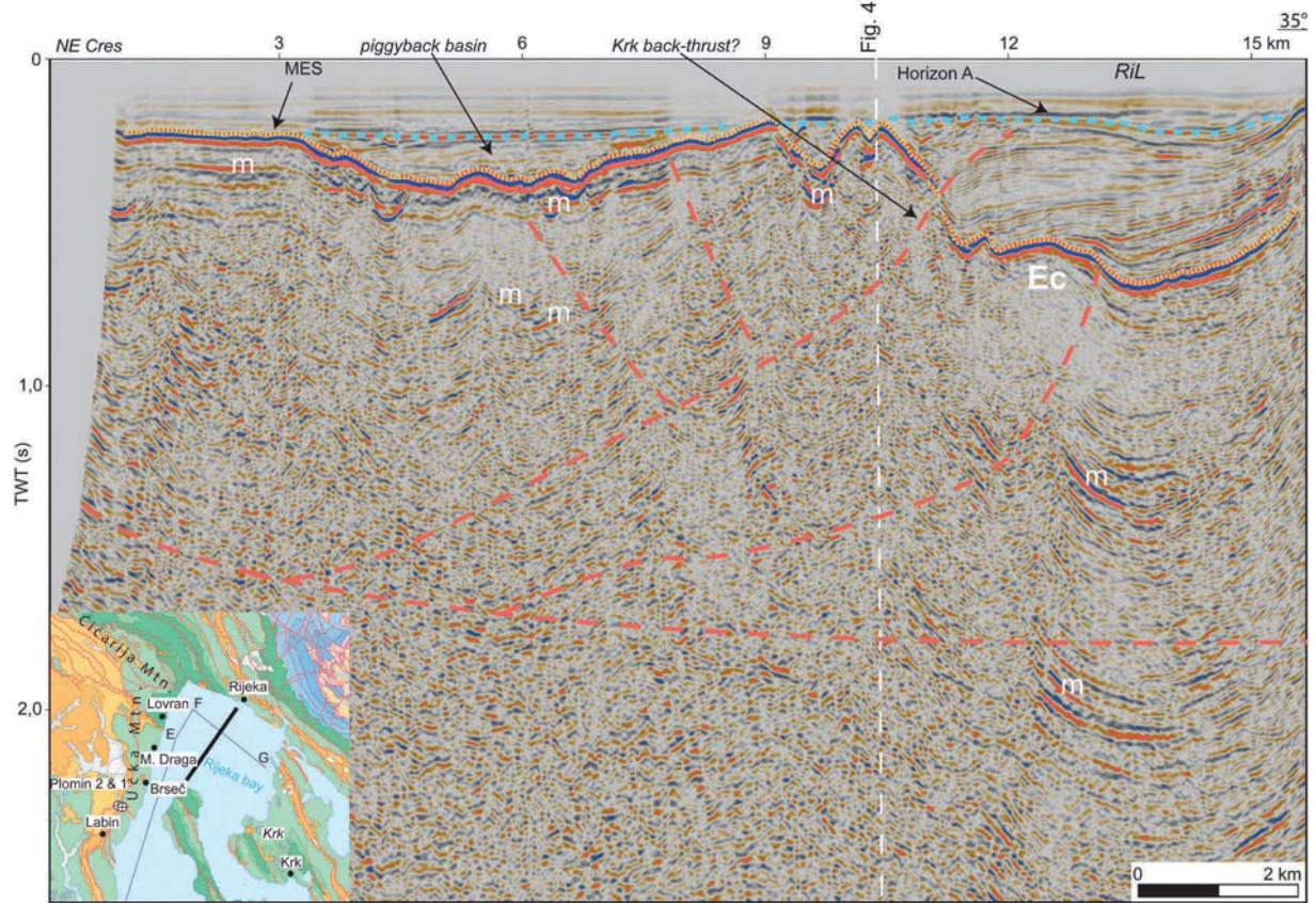
Fig. 11. Seismic profile with SW–NE direction, from the Cres to the Rijeka coasts. A deep basin is present between the Rijeka coast and the Krk back-thrust. The valley between 3 and 9 km is filled by a clinoform system downlapping the high amplitude reflector of the MES. The MES shows only a weak angular relationship with the underlying layers testifying that erosion clearly developed in the piggy-back basin. The deeper red dashed line, representing a SW verging thrust, has been interpreted on several profiles of the seismic dataset, as also in the northern part of the composite profile of Fig. 4. To the SW, the Cres offshore shows a sub-horizontal setting. (For interpretation of the references to colour in this figure legend, the reader is referred to the Web version of this article.)
