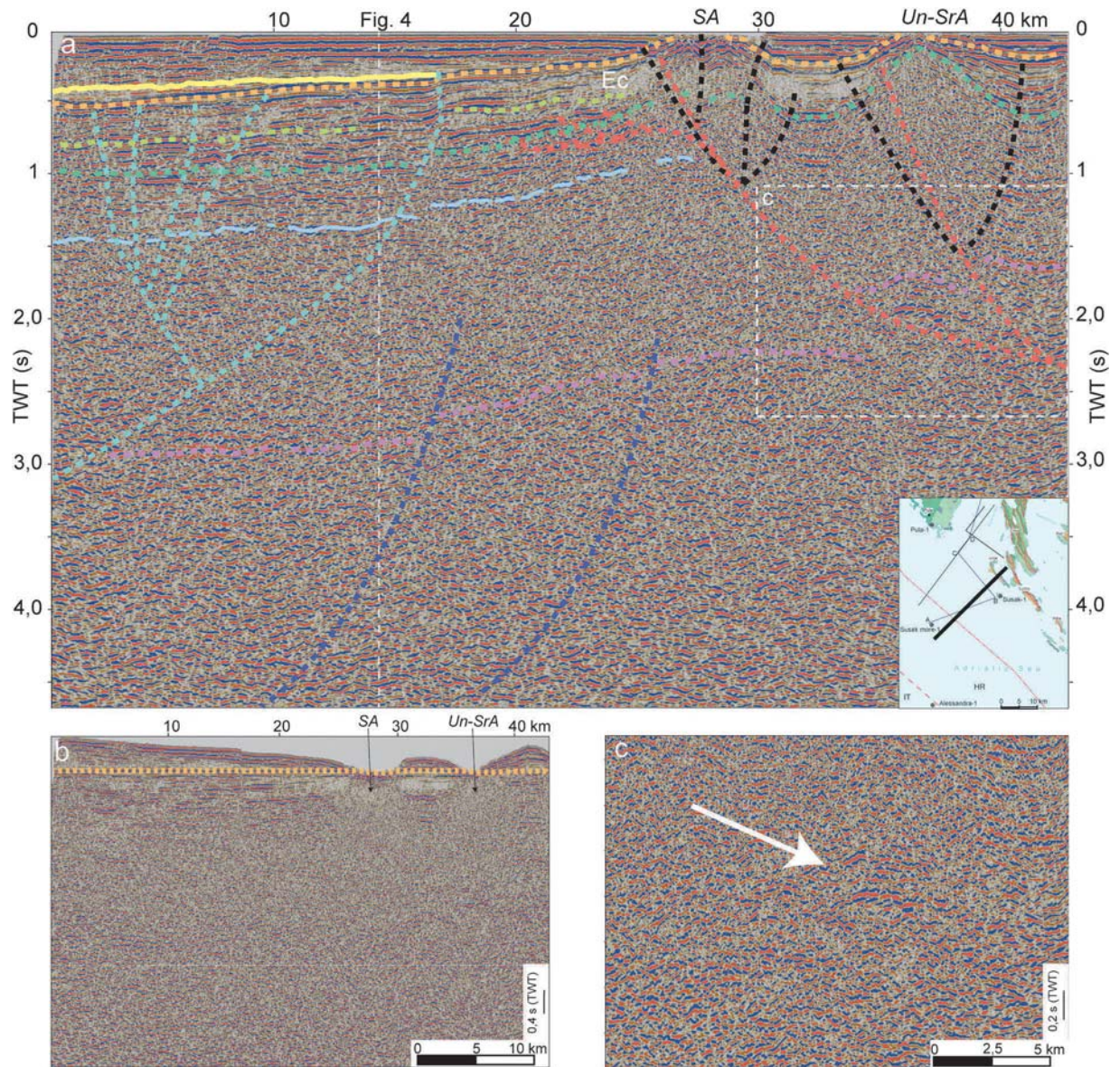
Fig. 8. Seismic profile through the Susak and the Unije-Srakane Anticlines. a) The left part of the profile shows the Pliocene tilting toward the Apennine Chain, which produced normal faults (light blue lines). Some of them likely reactivated the Triassic extensional faults (dark blue lines), generally affecting the deep Lower to Middle Triassic clastic sequence (below the pink horizon). The Susak and Unije-Srakane anticline structures (SA and Un-SrA) to the right were produced by Eocene thrusting (red lines) with syn-tectonic (Flysch?) strata (Ec). These structures were reactivated by post-Messinian transpressional deformation (black lines). We cannot exclude that they were originally isolated carbonate platforms. b) The section flattened on MES horizon gives an approximate image of the set-up in a post-Eocene compression/pre-foreland-tilting and Plio-Quaternary deformation time. c) White arrow indicates the faulted top of the Lower to Middle Triassic clastic sequence. (For interpretation of the references to colour in this figure legend, the reader is referred to the Web version of this article.)
