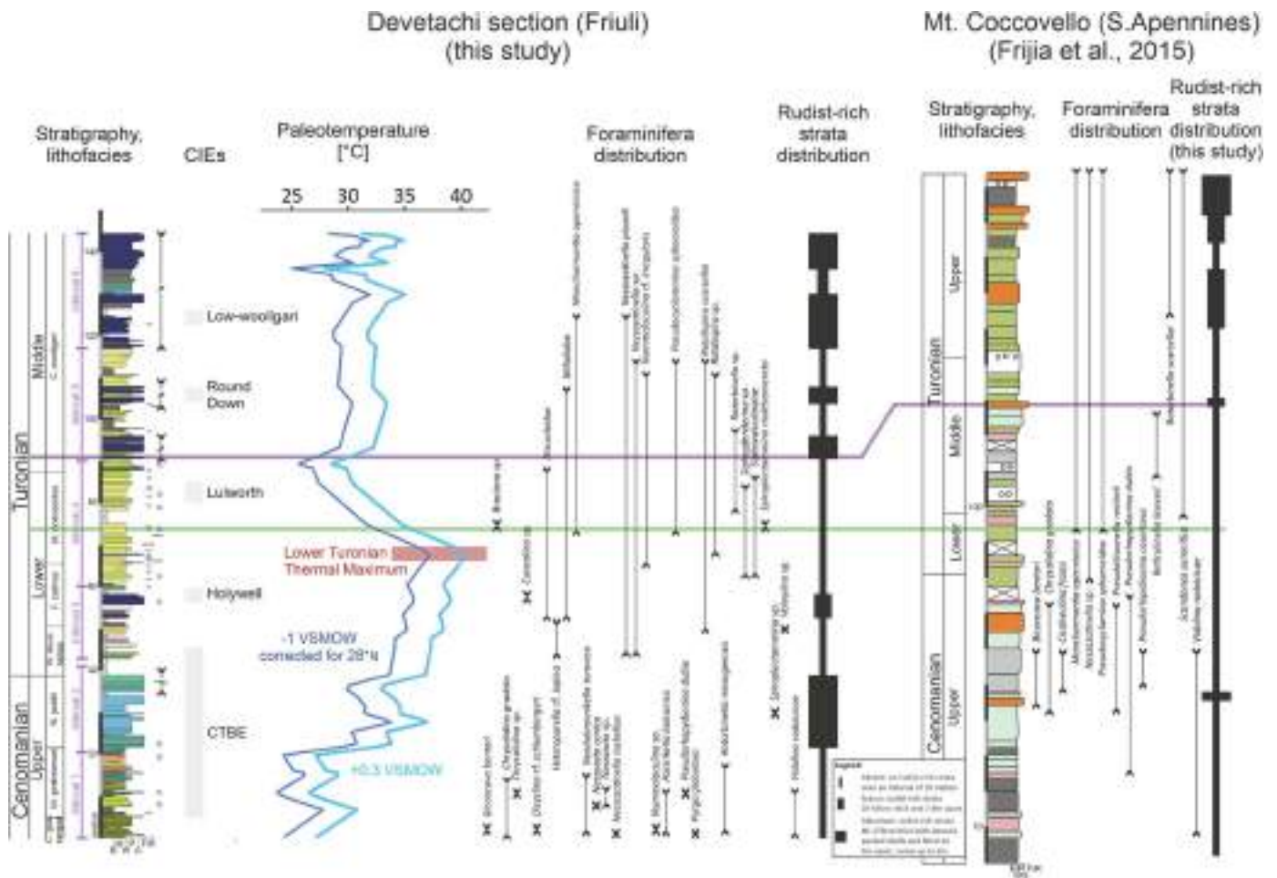
Fig. 9. Benthic foraminifera and rudists distribution in Devetachi section (Friuli Carbonate Platform, FCP) and Apennine carbonate platform (ACP, Frijia et al., 2015) across the upper Cenomanian-middle Turonian interval compared to the reconstructed temperature fluctuations. Foraminifera bioevents in the ACP are after Frijia et al. (2015). Black bars represent semiquantitative rudist abundance estimations (see text for details). Continuous green and purple lines mark the post-Cenomanian re-occurrence of high diversity foraminifera assemblages and rudist-dominated facies, respectively. Note that these bioevents occur after the Lower Turonian Thermal Maximum in both carbonate platform areas. (For interpretation of the references to colour in this figure legend, the reader is referred to the web version of this article.)
