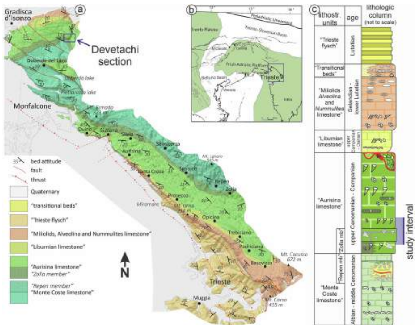
Fig. 1. Location and lithology of the studied area (modified from Consorti et al., 2021). 1a. Geological map of the Italian Karst (simplified from Jurkovšek et al., 2016). 1b. Cretaceous palaeogeographic map (after Picotti et al., 2019). 1c. Lithostratigraphic units and lithological columns of the studied area.
