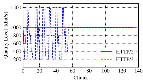
Fig. 14. Example sessions with 2 Mbit/s bandwidth ( BrowserTime-Video dataset).
