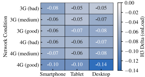
(a) onLoad.
