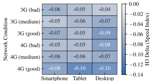
(b) SpeedIndex.
