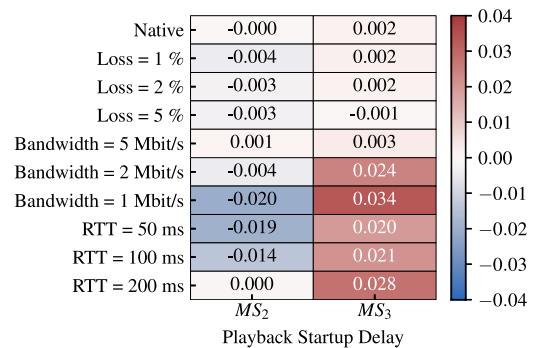
Fig. 12. Median Speedup per network condition ( BrowserTime-Video dataset). (For interpretation of the references to color in this figure legend, the reader is referred to the web version of this article.)
