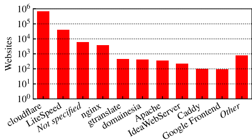
Fig. 3. Server in HTTP response (December 2020) ( HTTPArchive dataset).
