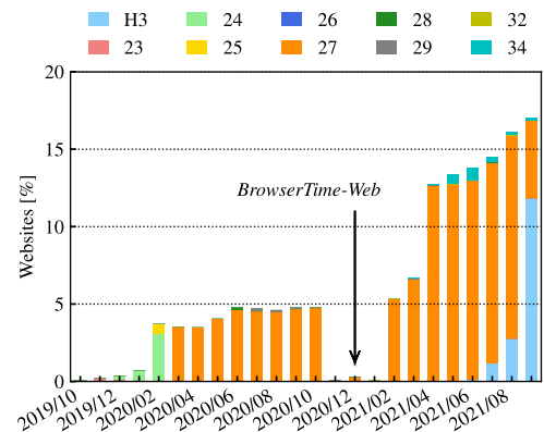
Fig. 2. Percentage of websites in HTTPArchive that announce support to HTTP/3, separately by IETF draft ( HTTPArchive dataset).
