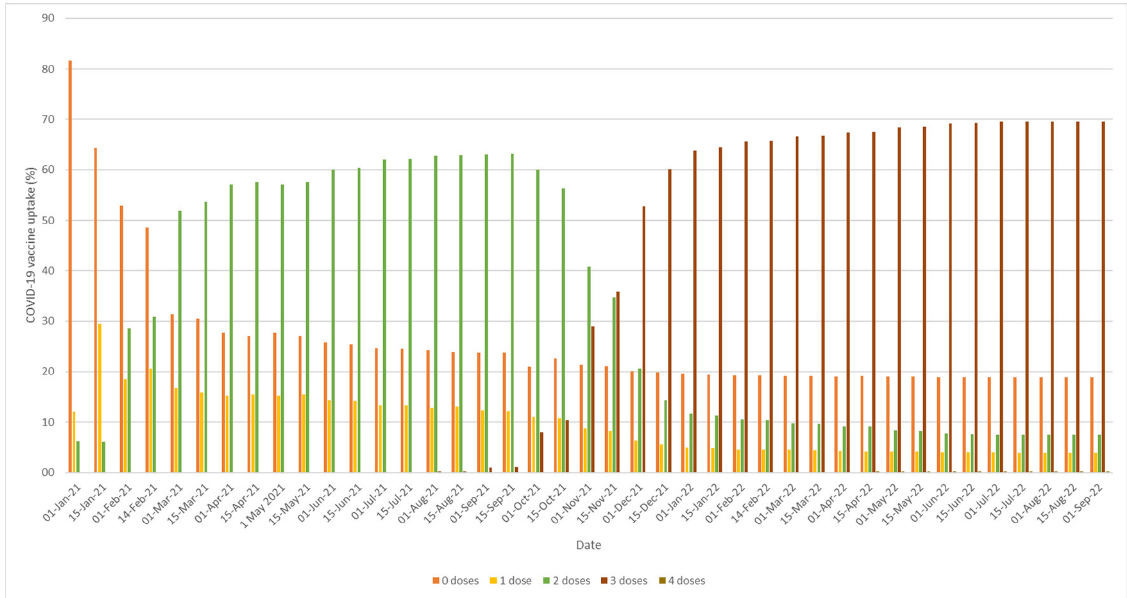
Supplementary Figure S1. COVID-19 vaccine uptake over time in health care workers from all four centres combined (N=5,432), by number of doses received.
