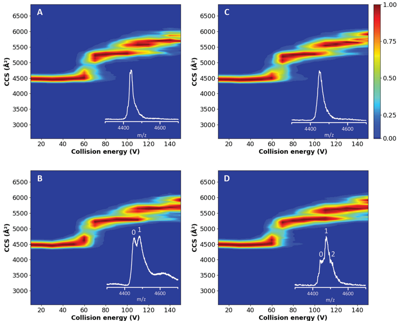
Fig. 3 CIU plots of untreated (A) and delipidated (C) hSA and of the untreated (B) and delipidated (D) hSA in complex with PFOA (1:10 protein:PFOA ratio). The ^{TW}CCS_{N_2} is plotted as a function of the trap collision energy and the intensity is shown using a colour scale (red is 100% and blue 0%). The insets show the peaks selected (15+ charge state) for extraction of the ^{TW}CCS_{N_2} at a trap collision energy of 60 V. Arrival times were extracted from the whole peak, including salt adducts and complexes (where appropriate).
