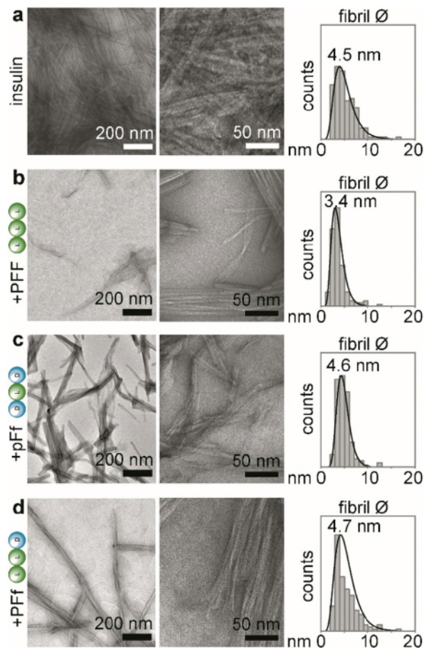
Fig. 2 TEM analyses of insulin fibrillation inhibition, showing TEM micrographs at lower (left panels) and higher (middle panels) magnification, and statistical distribution of fibrils' diameters with the reported median value (right panels, n = 150 counts). (a) insulin alone; (b) insulin + PFF; (c) insulin + pFf; (d) insulin + PFf.
