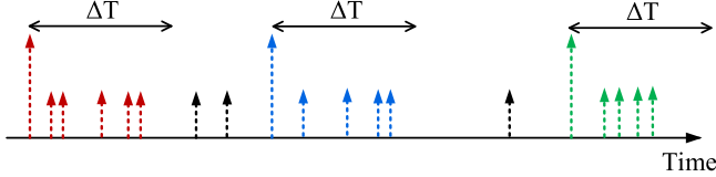
Fig. 4. Support domain learning: a flow to a core domain triggers a new observation window, used to learn the support domain set S_c .
