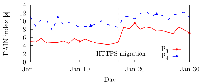
Fig. 13. PAIN index for www.poste.it over 1 month ( RealWorld ).
