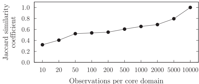
Fig. 10. Support domains for increasing number of observations per core domain, compared to 10,000 observations ( RealWorld ).
