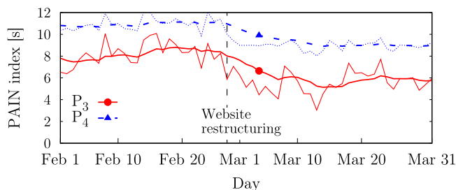
Fig. 14. PAIN index trend for www.repubblica.it before and after website restructuring ( RealWorld ).
