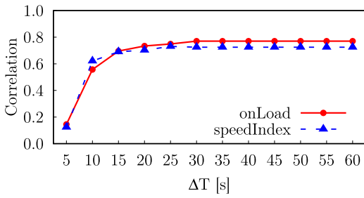
Fig. 5. Spearman Correlation of P_3 with onLoad and SpeedIndex when varying \Delta T (SynthTypical dataset).
