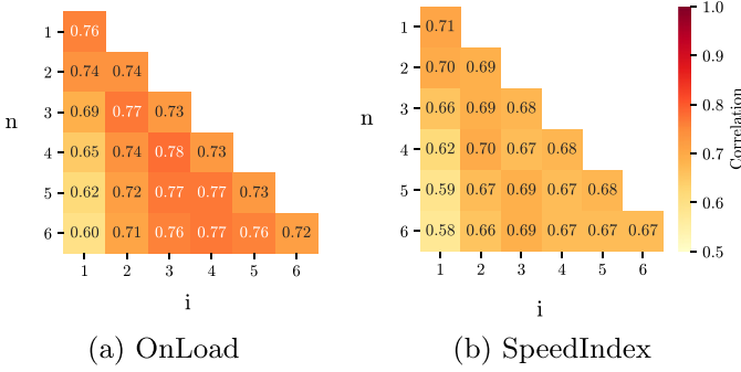
Fig. 6. Correlation of PAIN index with onLoad and SpeedIndex when varying the number of groups n (SynthTypical dataset).
