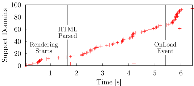
Fig. 2. Support domain flows for a visit to www.bbc.co.uk . The browser contacted 94 support domains (y-axis) during 6 seconds (x-axis). Notable browser events are reported as vertical lines.
