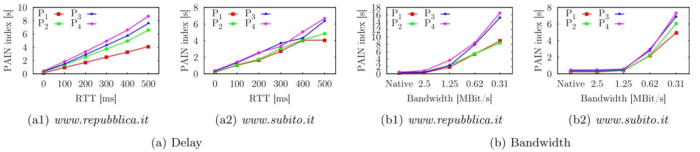
Fig. 7. Median value of PAIN index when varying delay and bandwidth (SynthDegraded dataset).
