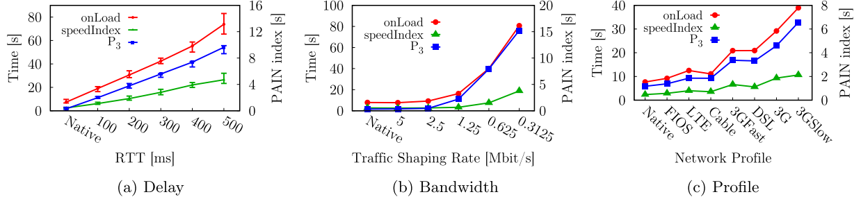
Fig. 8. www.repubblica.it onLoad, SpeedIndex and P_3 for various setups (SynthTypical and SynthDegraded datasets). (For interpretation of the references to colour in this figure legend, the reader is referred to the web version of this article.)
