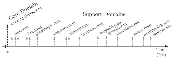
Fig. 1. Sample of flows in a visit to www.nytimes.com . We use the time to contact support domains to monitor performance.
