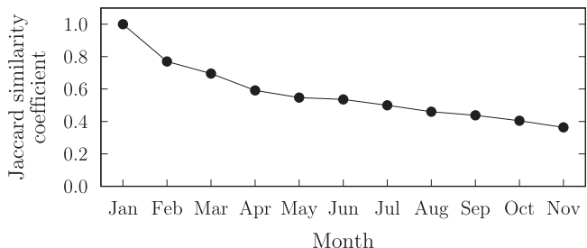
Fig. 11. Support domains over the months of a year ( RealWorld ).
