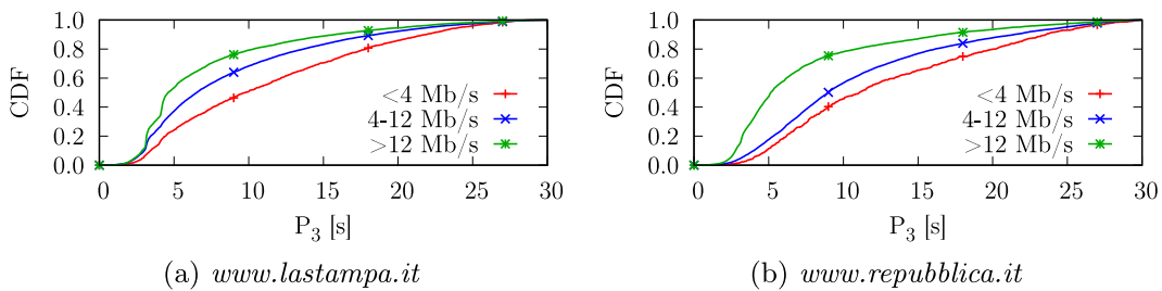
Fig. 12. Distribution of PAIN P_3 index according to the access-link capacity for all visits in RealWorld dataset.
