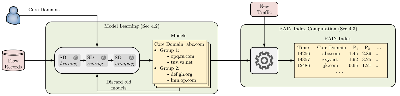
Fig. 3. Architecture of PAIN. It learns and clusters support domains using flow records and a list of target core domains. The resulting groups are used to estimate performance.
