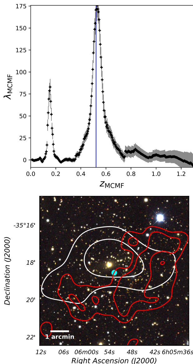
Figure A1. Top: Richness as a function of redshift for the Planck candidate PSZ-SN3 J0605-3519. Two richness peaks at z_{\text{MCMF}} = 0.15 and z_{\text{MCMF}} = 0.52 are evident. Bottom: Pseudo-colour image from DES g, r, i cutouts around the Planck candidate coordinates, marked by a cyan dot. Contours are from the galaxy density maps of the counterpart at z_{\text{MCMF}} = 0.15 (white) and at z_{\text{MCMF}} = 0.52 (red).
