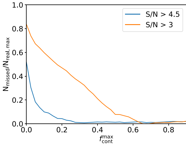
Figure 10. Estimate of the fractional incompleteness versus the f_{\text{cont}} threshold f_{\text{cont}}^{\text{max}} for the S/N>4.5 ( f_{\text{SZE-cont}} = 8.5 per cent) and S/N>3 ( f_{\text{SZE-cont}} = 51 per cent) confirmed cluster samples, shown with blue and orange lines, respectively. The contamination of the resulting cluster catalogue is given by f_{\text{SZE-cont}} f_{\text{cont}}^{\text{max}} (see Section 4.4.1 and Table 1).
