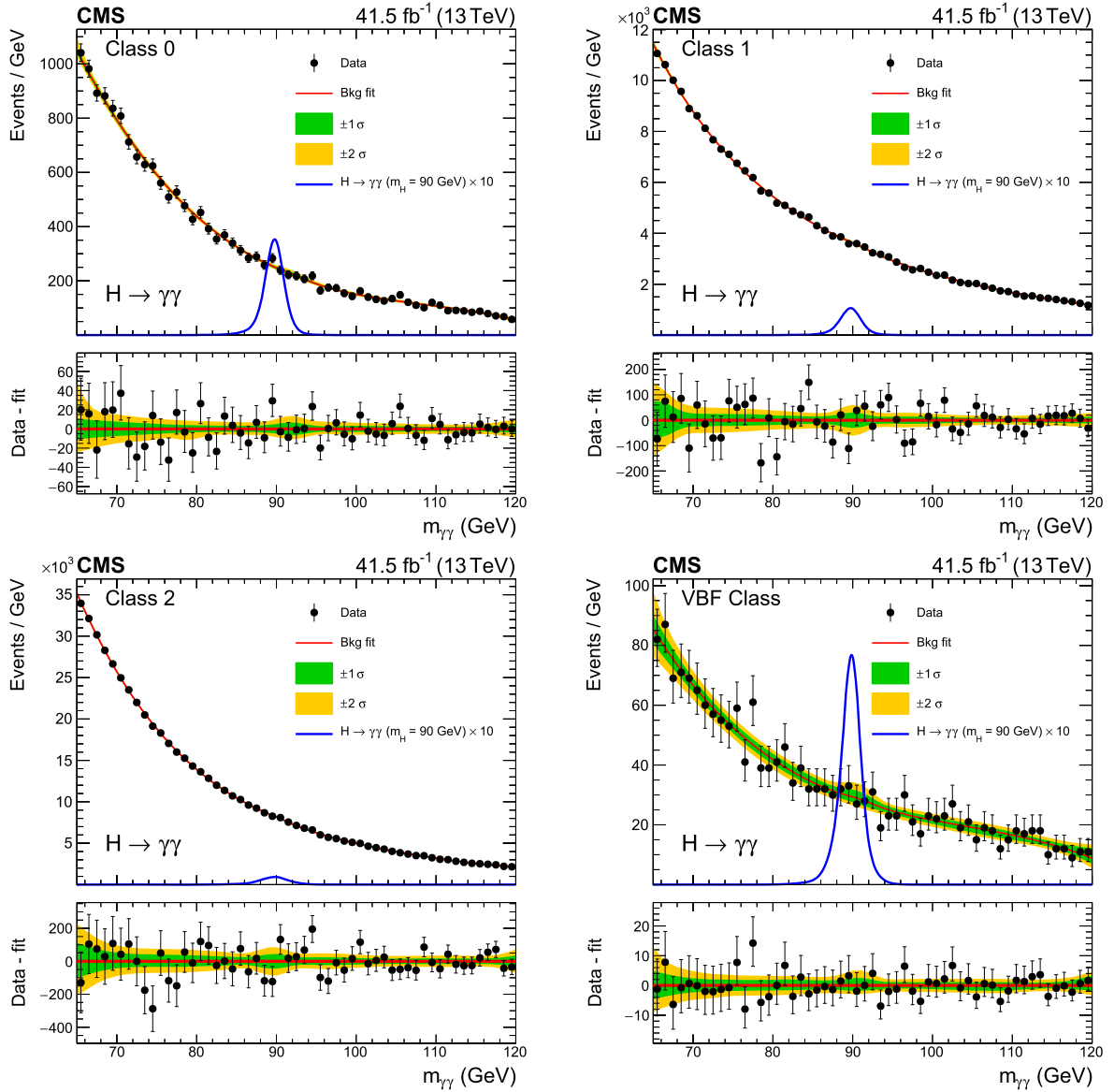
Fig. 3. Background model fits using the chosen background model parametrization to the 2017 data in the four event classes. The corresponding signal model for each class and m_H = 90 GeV, multiplied by 10, is also shown. The one- and two- \sigma bands reflect the uncertainty in the background model normalization associated with the statistical uncertainties of the fits, and are shown for illustration purposes only. The difference between the data and the background model is shown in the lower panels.
