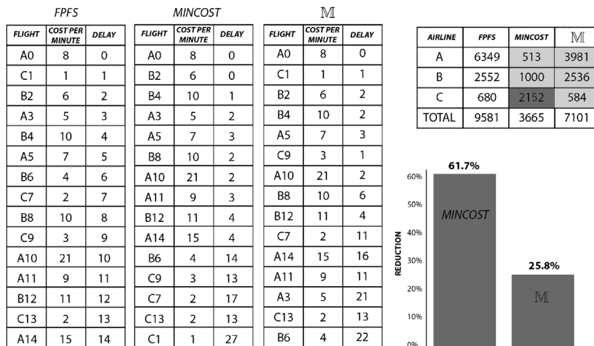
Fig. 1. Comparison between the MINCOST and mechanism M.
