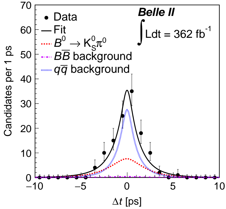
FIG. 1: Distributions of \Delta t with fit projections overlaid for both signal and background candidates satisfying the criteria 5.27 < M'_{bc} < 5.29 \text{ GeV} , -0.15 < \Delta E < 0.10 \text{ GeV} , and C'_{\text{BDT}} > 0.0 . The solid curve represent the fit projection, while various fit components are explained in the legends.
