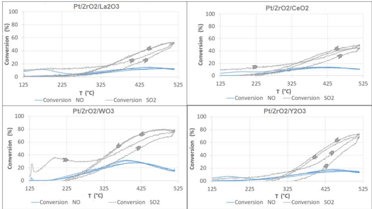
Figure 7: Comparison of conversion curves (NO to NO 2 and SO 2 to SO 3 ) as a function of temperature over Pt/doped-ZrO 2 catalysts.
