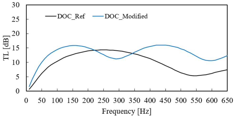
Figure 9: TL comparison, reference DOC vs modified one.
