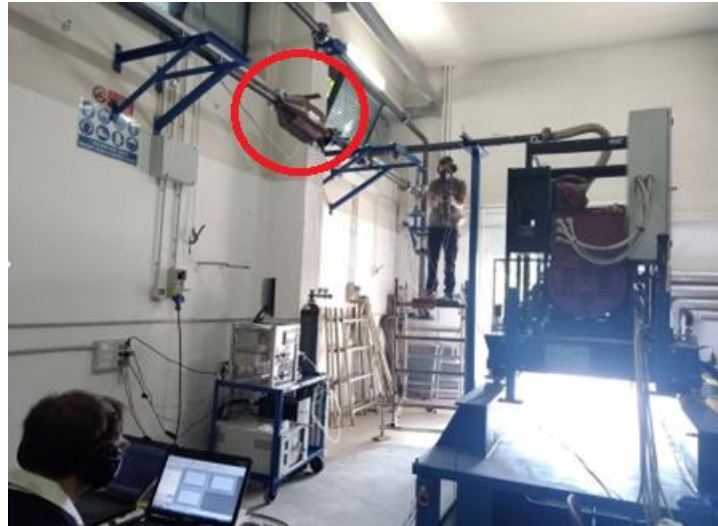
Figure 5: Diesel Genset mockup, DOC converter rounded in red.
