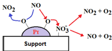
Figure 6: Eley-Rideal mechanism proposed for \text{NO} oxidation over Pt catalysts (Li et al., 2010).
