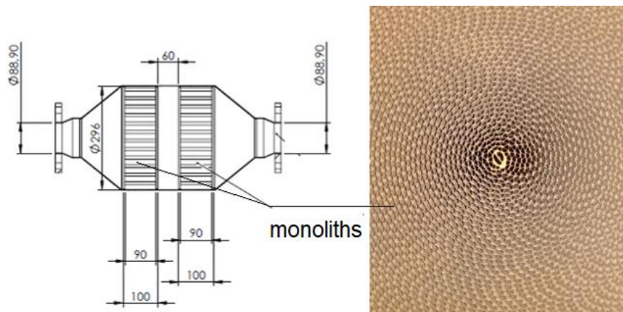
Figure 8: Scheme of the DOC converter and detail of the honeycomb structure.
