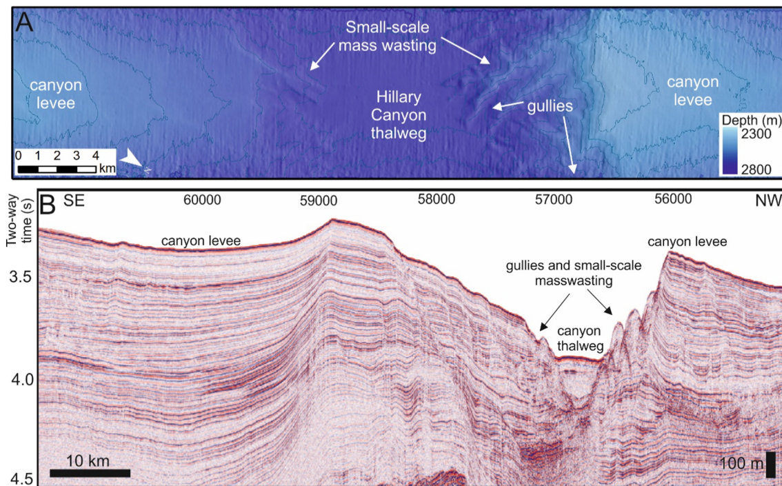
Fig. 5. A. Morphology of the Hillary Canyon thalweg. Hillshaded bathymetry is gridded at 50 m. Contour spacing is 50 m. Location of (A) shown in Fig. 1B. B. Single channel seismic line IT17RS303 showing cross-section through the Hillary Canyon thalweg and canyon levees.
