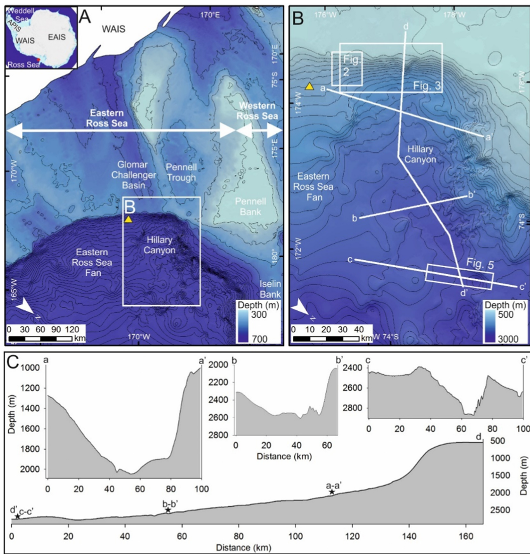
Fig. 1. A. Study area in the Ross Sea. White box shows location of (B). Bathymetric data is International Bathymetric Chart of the Southern Ocean (IBCSO, Arndt et al., 2013). Yellow triangle is position of cores RS14-BC3 and RS14-C3. Contour spacing is 200 m. B. Hillary Canyon regional bathymetry taken from IBCSO. White lines indicate positions of along and down-slope profiles shown in (C). White boxes show locations of Figs. 2, 3 and 5. Yellow triangle is position of cores RS14-BC3 and RS14-C3. C. Along and down-slope profiles across the Hillary Canyon derived from bathymetry using IBCSO. Stars highlight position of along-slope profiles shown in (B).
