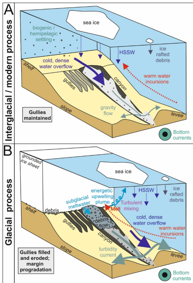
Fig. 9. Schematic of canyon head processes operating in glacial vs interglacial settings. A. Interglacial/modern conditions where gravity flows are generated by fine grained biogenic/hemipelagic material that is resuspended by energetic cascading cold, dense water. B. Glacial conditions where energetic turbidity currents may be generated by either: the release of subglacial meltwater; meltwater generated by intruding warm currents at the ice front; slope failure. HSSW is High Salinity Shelf Water.
