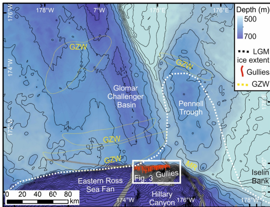
Fig. 8. Inferred ice position at Last Glacial Maximum. Background bathymetric data is International Bathymetric Chart of the Southern Ocean (IBCSO). Contour spacing is 50 m. Hillshaded bathymetry from ANTSS expedition gridded at 50 m cell size. White dashed line is inferred ice extent at LGM taken from Halberstadt et al. (2016). GZW is Grounding Zone Wedge position taken from Halberstadt et al. (2016). MR is moraine ridge. Red lines are gully positions.
