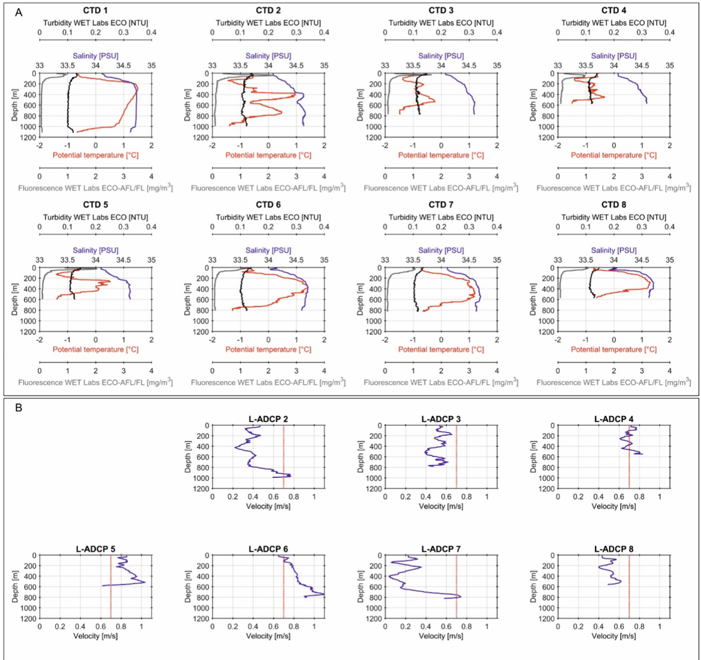
Fig. 7. Oceanographic measurements at the head of the Hillary Canyon, Ross Sea. A. Conductivity Temperature Depth (CTD) profiles with fluorescence and turbidity sensor data. Location of CTD profiles are shown in Fig. 6C. B. Lowered-Acoustic Doppler Current Profiler data. Positions are shown in Fig. 6C. Red dashed line marks 0.7 m/s for comparison in all profiles.
