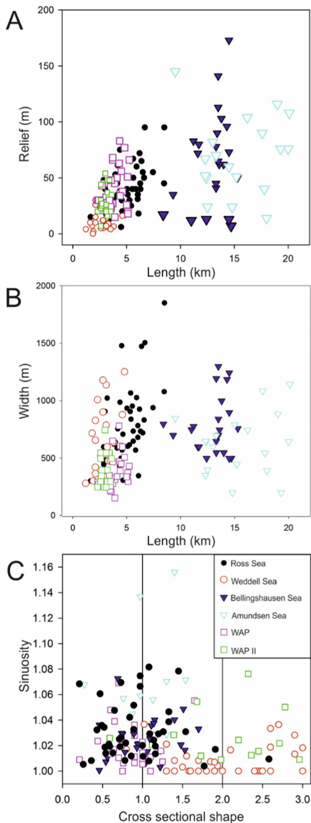
Fig. 10. Antarctic gully morphometric parameters. A. Gully length vs gully relief. B. Gully width vs gully length. C. Gully sinuosity vs cross sectional shape. Data from the Weddell Sea, Bellingshausen Sea, Amundsen Sea, Western Antarctic Peninsula (WAP) taken from Gales et al. (2013). Ross Sea data from this study. For calculations of gully parameters, see SM. Fig. 1.
