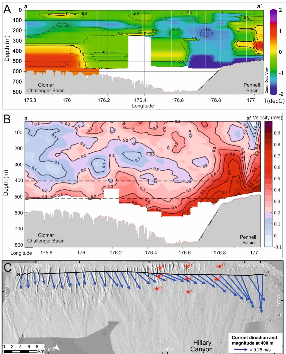
Fig. 6. Oceanographic measurements along profile a-a'. A. Temperature data from 20 expendable BathyThermograph (XBT) profiles along profile a-a' located in (C). B. Current velocity data from Acoustic Doppler Current Profiler along profile a-a' located in (C). C. Hillshaded bathymetric data gridded at 50 m at the head of the Hillary Canyon, Ross Sea. Black line locates profile a-a' shown in (A) and (B). Blue lines are current vectors indicating current direction at 400 m water depth along dashed line in (B). Red stars locate eight Conductivity Temperature Depth profiles shown in Fig. 7A.
