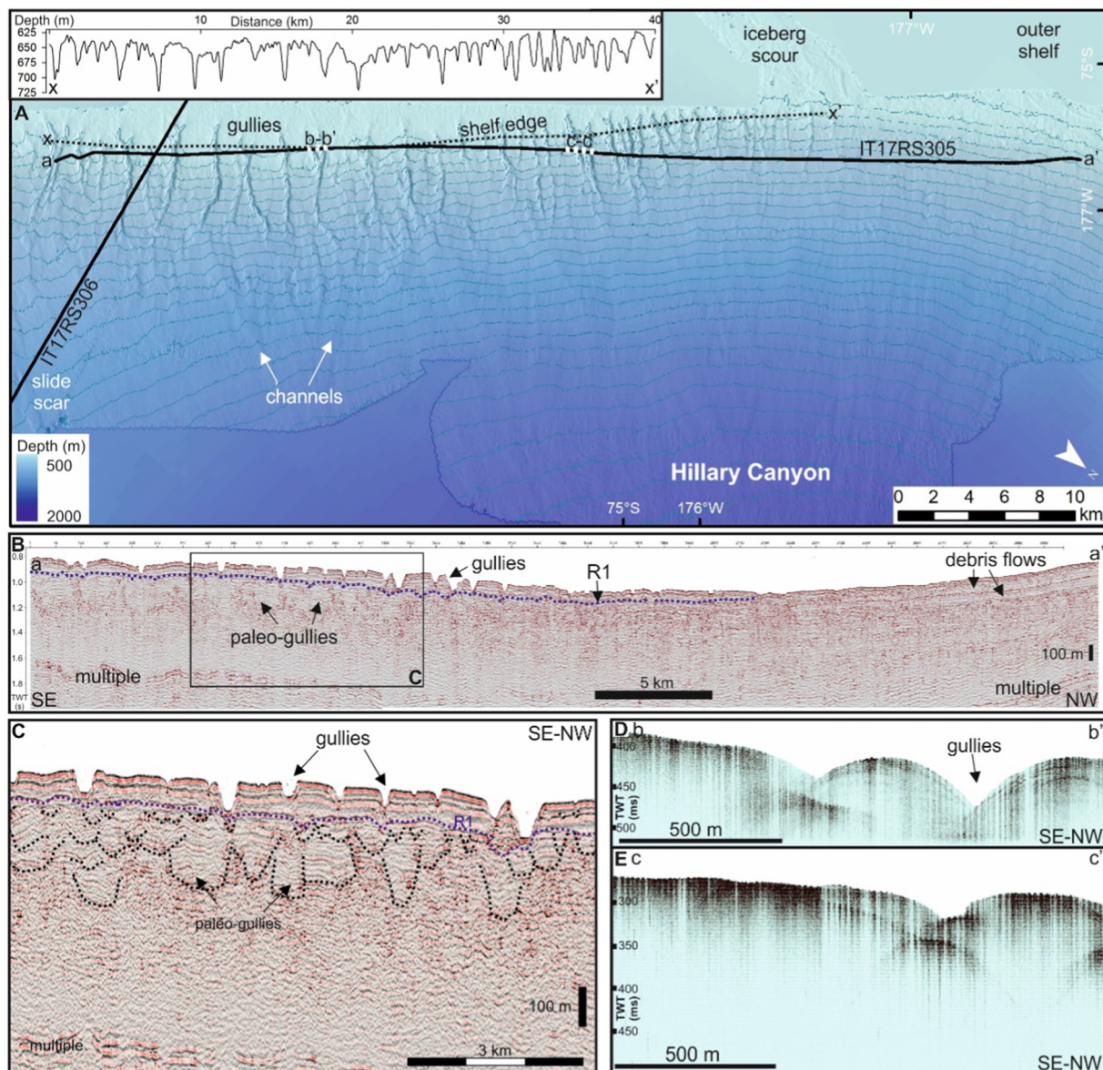
Fig. 3. A. Morphology at the head of the Hillary Canyon, Ross Sea. Hillshaded bathymetry gridded at 50 m cell size. Contour spacing is 50 m. Background bathymetric data is International Bathymetric Chart of the Southern Ocean (IBCSO). Black lines mark location of single channel seismic lines IT17RS305 in (B) and IT17RS306. Black dashed line x-x' locates along-slope profile in (A). White dashed lines b-b' and c-c' locate sub-bottom profiles in (D) and (E). B. Single channel seismic line IT17RS305. Black box locates (C). C. Zoom-in of seismic line IT17RS305 located in (B). D. Unmigrated sub-bottom profile located in (A). E. Unmigrated sub-bottom profile located in (A).
