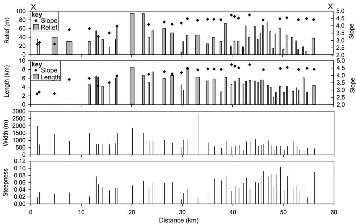
Fig. 4. Gully morphometric parameters along profile X-X' located in Fig. 3A. Width of bars in top two panels correspond to gully width. Black diamonds correspond to average slope gradient ( ^{\circ} ) of the upper slope with distance parallel to the shelf edge.
