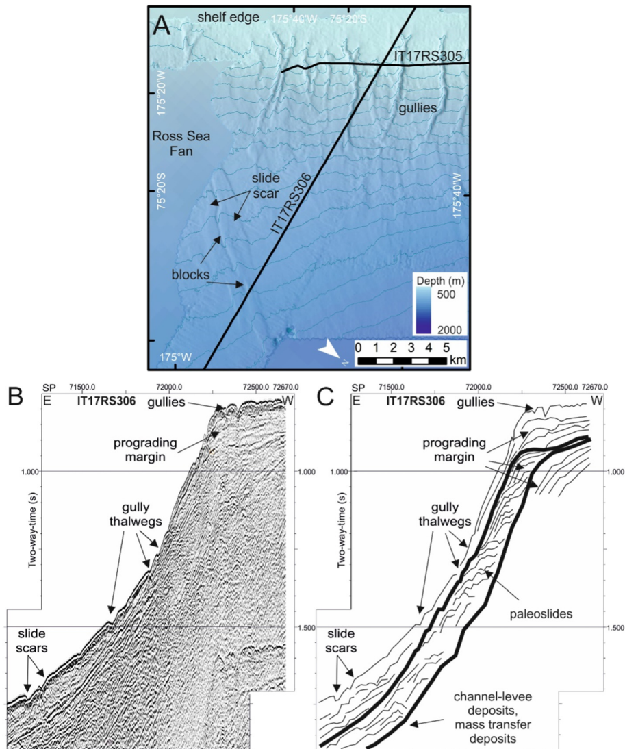
Fig. 2. Submarine slide morphology and prograded continental margin at the mouth of the Glomar Challenger Basin. A. Slide morphology. Hillshaded bathymetry is gridded at 50 m. Regional bathymetry is from IBCSO. Contour spacing is 50 m. Black lines mark location of single channel seismic lines IT17RS305 and IT17RS306. B. Seismic line IT17RS306 (near trace). C. Interpretation of seismic line IT17RS306 (near trace).
