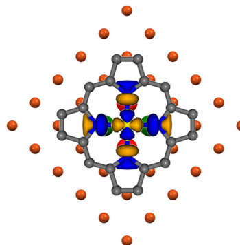
Fig. 8 Superposition of the {}^{\text{pmc}}\sigma^* 12b_{1g} -based MO (LUMO+2) 37 3D CP to the {}^{\text{nn}}\text{Cu}_{\text{ffa}}^{\text{S}} 4s AOs SALC of symmetry b of the bulk terminated Cu(100). Ni–N bonds are aligned with the \langle 001 \rangle directions. Large red and green spheres represent \text{Cu}^{\text{S}} 4s AOs and corresponding different phases.
