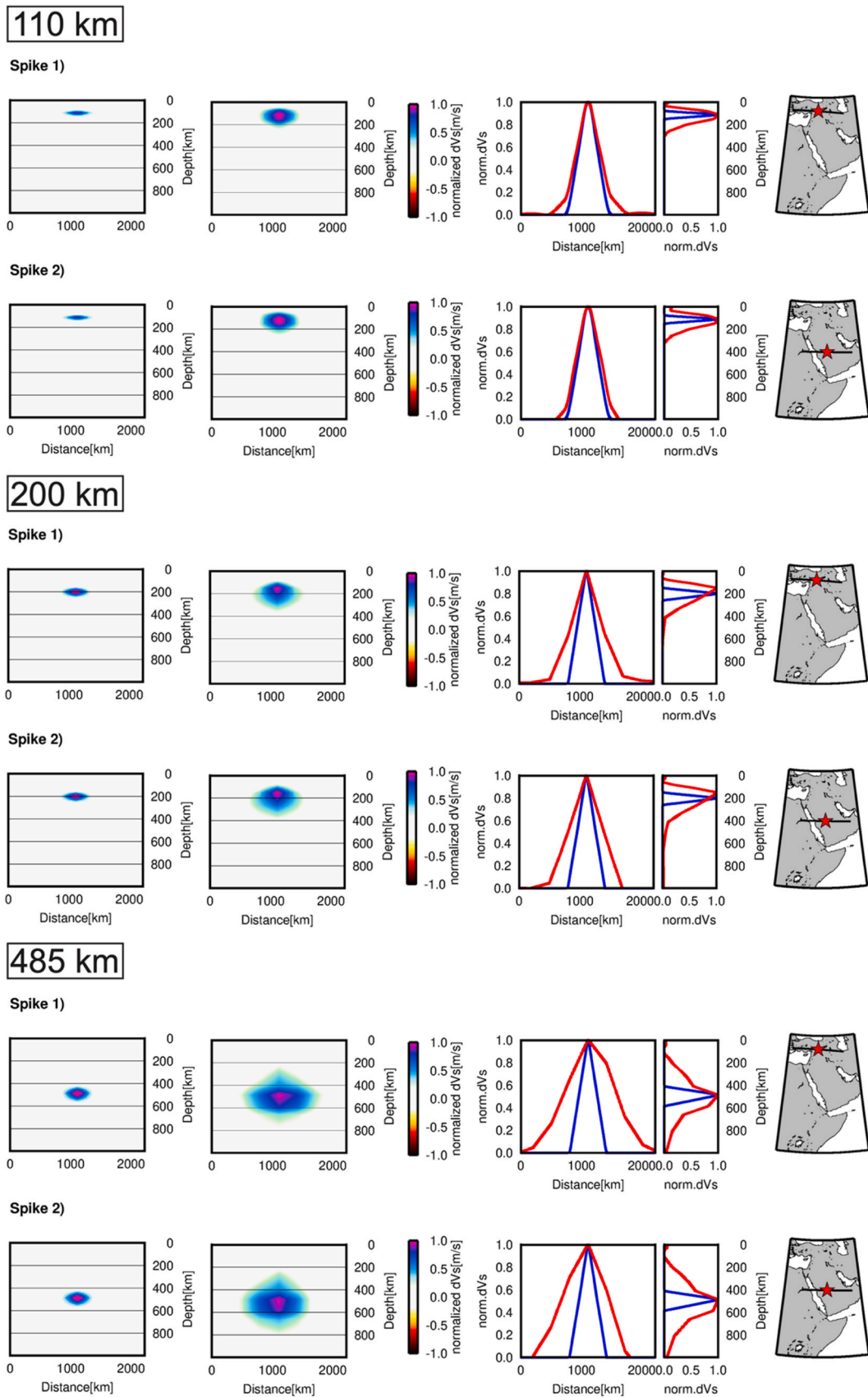
Fig. 5. Spike resolution tests. Spikes' location is shown on the map on the right as red stars. The input spikes are placed at 110, 200 and 485 km depth. For each spike we plot a vertical cross-section through the input (first panel) and output (second panel) models. The orientation of the profile is shown on the map in black. The third and fourth panels indicate horizontal and vertical 1-D S-wave anomaly profiles along the cross-section. Input profiles are shown in blue, and output in red. All S-wave velocity anomalies are normalized to the maximum.
