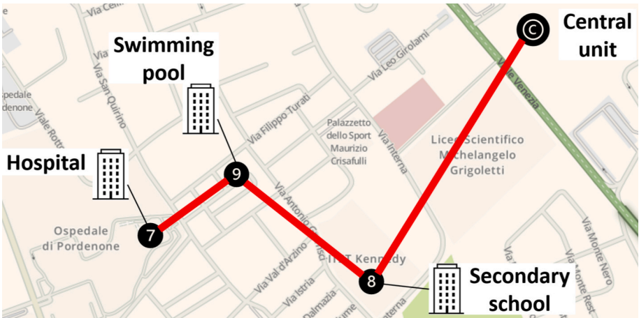
Fig. 16. Optimal economic solution: DHN pipeline connections between buildings 7, 9, 8, and central unit.
