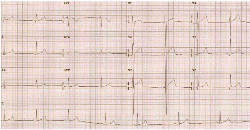
FIGURE 1 Electrocardiogram of a cyclist with LVEDD 63 mm and LVEF 50% at transthoracic echocardiogram (A). ECG of a 50 years old man with DCM (FLNC pathogenic variant) (B). Note the low voltages and the TWI in the inferolateral leads.
