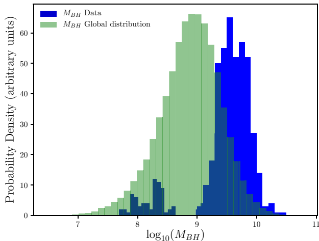
Figure A1. Histograms showing that our lag measurements primarily sample the high-mass end of the black hole mass distribution predicted by equation (A2). This is expected since we are primarily sensitive to long lags. The data in blue was obtained using the lag estimated from the R-L relation listed in Hoormann et al. (2019) and the line velocities from the RMS spectra for each source. These are then used to compute a mass using the virial relation (equation 1). The green distribution is the prediction of the black hole mass distribution using equation (A2) and the absolute i -band magnitudes for each source.
