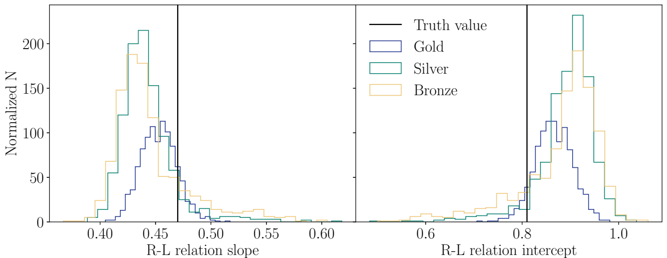
Figure 12. Best-fitting R-L relation slopes ( \frac{\log_{10}(\text{days})}{\log_{10}(\text{erg}\cdot\text{s}^{-1})} ) and intercepts [ \log_{10}(\text{days}) ] computed using a subsample of sources from each cut group. These histograms contain 1000 iterations of the fitting procedure. The cuts have an obvious effect on the quality of the R-L relation recovery with the gold standard fits being centred around the truth value for the slope and closest of the three groups for the intercept. Next most reliable is silver and then bronze as expected. All three distributions are offset from the truth value with regards to the intercept; this is likely due to the positive offset seen in the simulation results and may be compensated for if well understood. Note that the mean uncertainties in the intercept measurements are approximately 0.034 for all cuts, with the average uncertainty in the intercept being 0.070, 0.077, and 0.086 for the gold, silver, and bronze level cuts, respectively.
