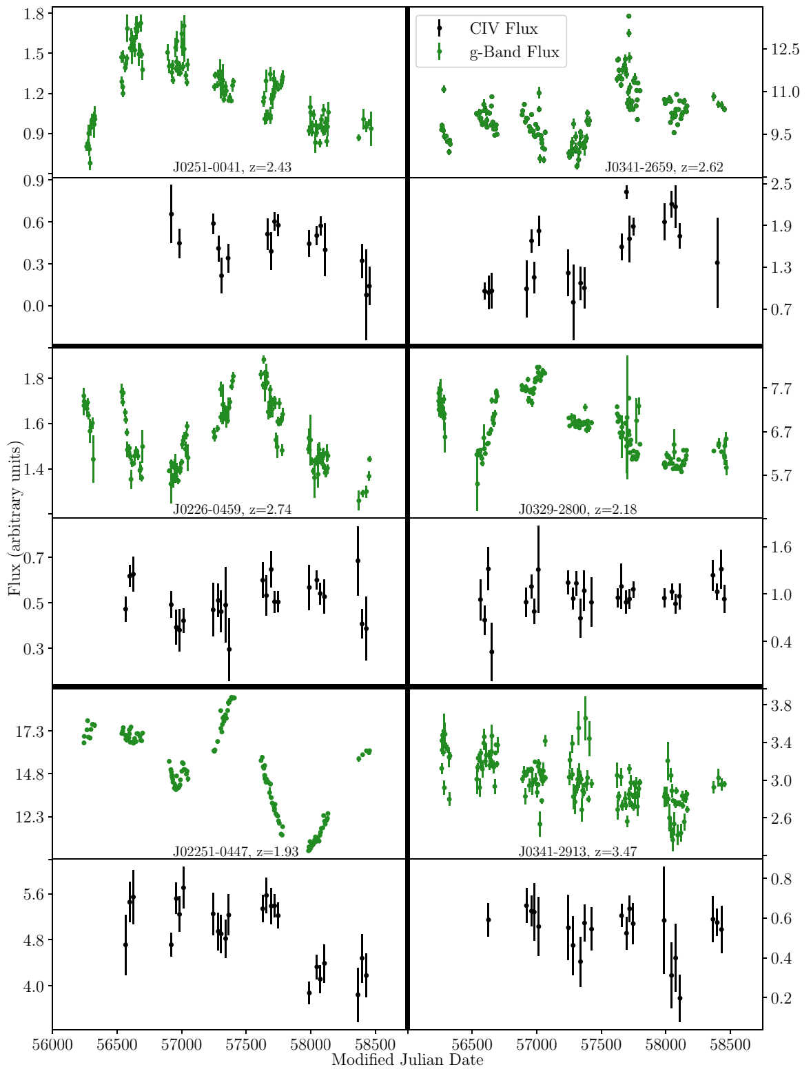
Figure 1. Representative light curves from the OzDES RM sample. CIV emission line light curves shown in black, with g-band photometric light curves shown in green. The photometric light curves contain seven seasons of data with approximately weekly cadence. These are accompanied by spectroscopic light curves containing 5-6 seasons of approximately monthly cadence.
