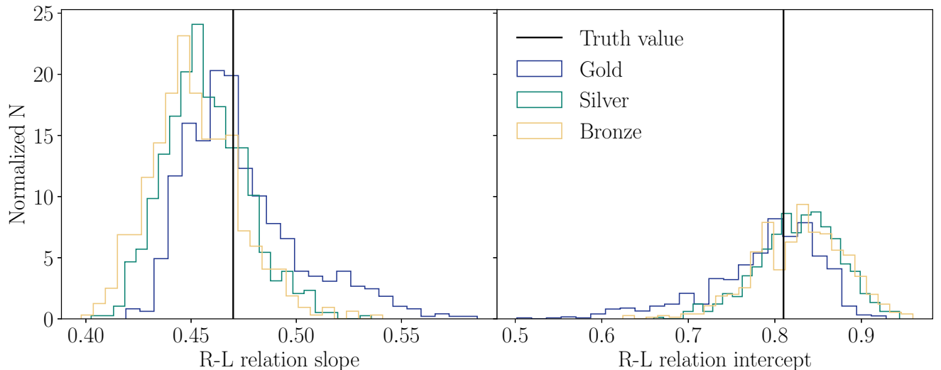
Figure B1. Best-fitting R-L relation slopes ( \frac{\log_{10}(\text{days})}{\log_{10}(\text{erg. s}^{-1})} ) and intercepts [ \log_{10}(\text{days}) ] computed using a subsample of sources from each cut group, with corrections for each based on the average offset shown in Table 2. We can see that the biases seen in Fig. 12 are greatly reduced. This indicates that using these simulations to account for biases can be effective.
