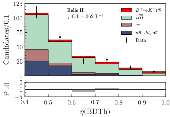
FIG. 19. Observed yields and fit results in bins of \eta(\text{BDTh}) as obtained by the HTA fit, corresponding to an integrated luminosity of 362 \text{ fb}^{-1} . The yields are shown for the B^+ \rightarrow K^+\nu\bar{\nu} signal and the three background categories ( B\bar{B} decays, c\bar{c} continuum, and light-quark continuum). The pull distribution is shown in the bottom panel.
