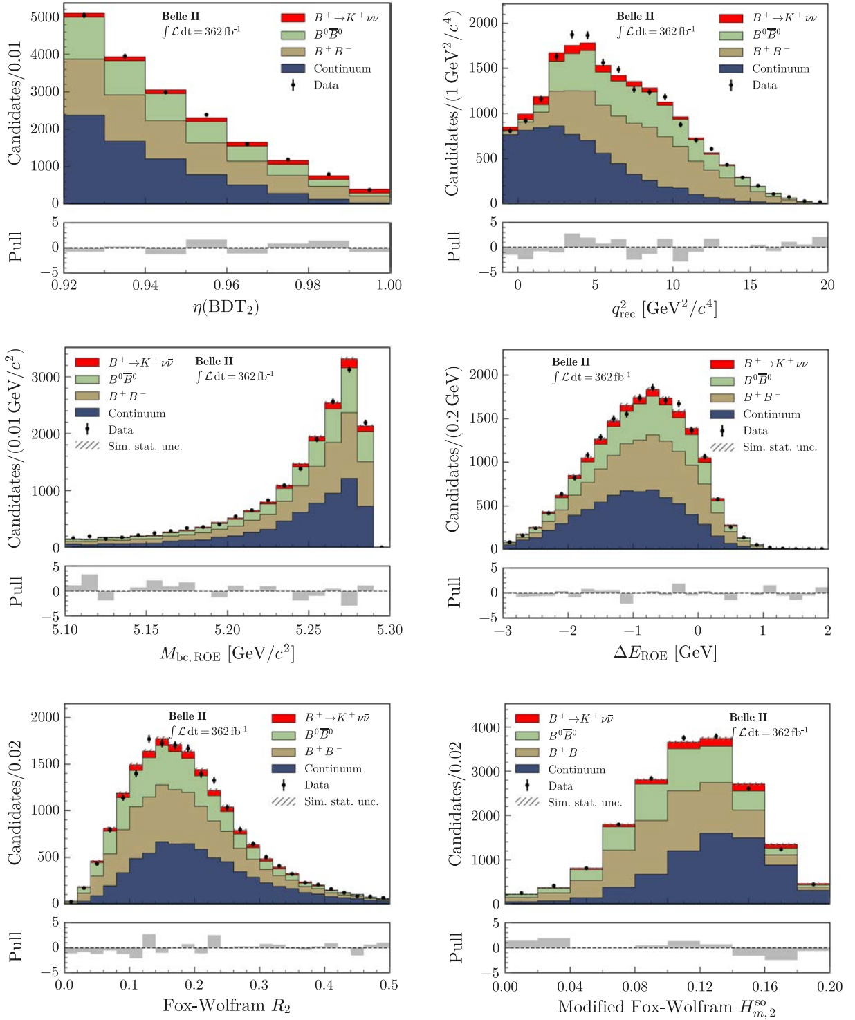
FIG. 17. Distributions of \eta(\text{BDT}_2) , q_{\text{rec}}^2 , beam-constrained mass of the ROE M_{\text{bc,ROE}} , \Delta E_{\text{ROE}} , Fox-Wolfram R_2 , and modified Fox-Wolfram H_{m,2}^{\text{so}} in data (points with error bars) and simulation (filled histograms) shown individually for the B^+ \rightarrow K^+ \nu \bar{\nu} signal, neutral and charged B -meson decays, and the sum of the five continuum categories in the ITA. Events in the full signal region, with \eta(\text{BDT}_2) > 0.92 , are shown. Simulated samples are normalized according to the fit yields in the ITA. The pull distributions are shown in the bottom panels.
