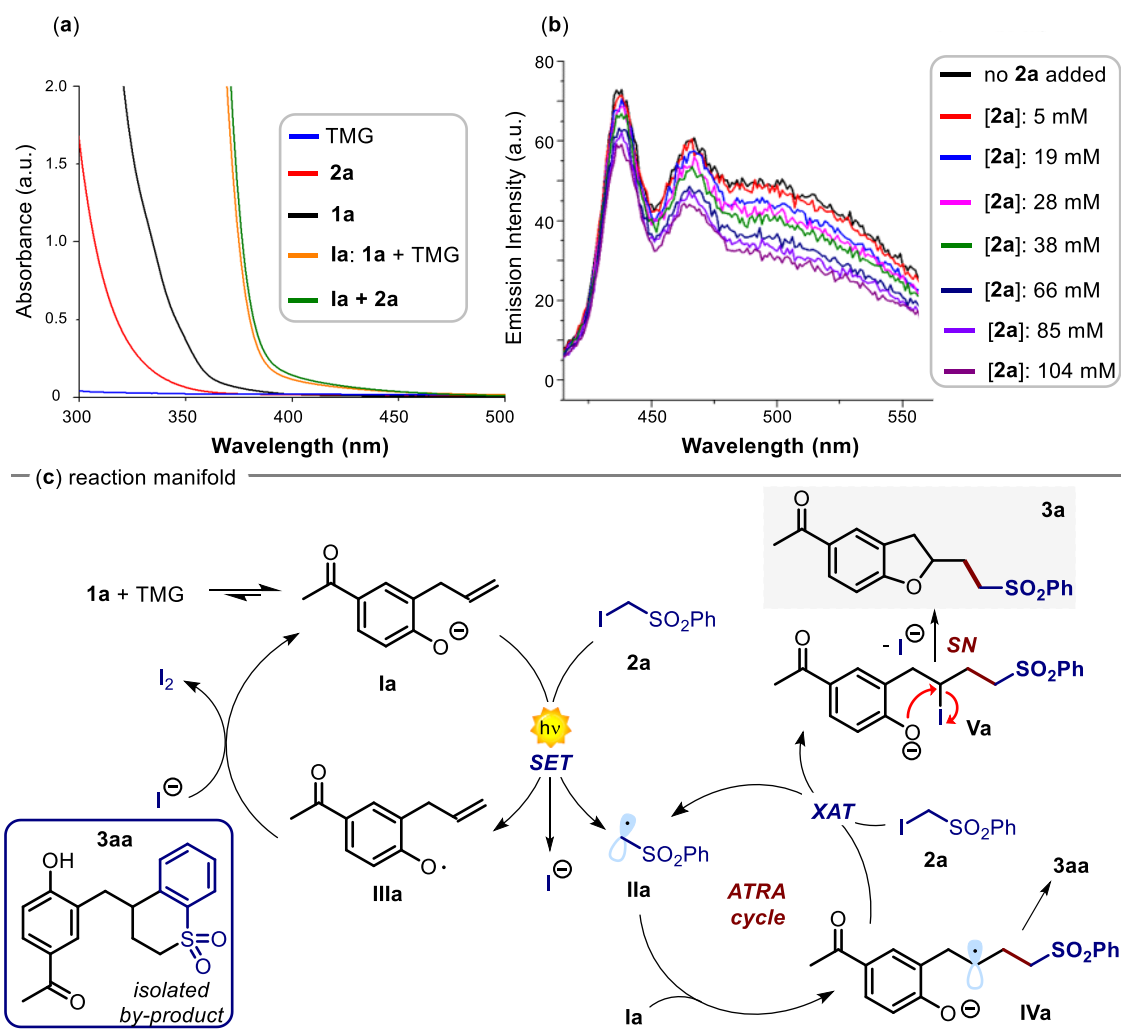
Figure 2. (a) Optical absorption spectra recorded in 1,2-dichlorobenzene: [1a] = 0.01 M (black line); [2a] = 0.01 M (red line); [TMG] = 0.01 M (blue line). (b) Quenching of the phenolate Ia emission ( [1a] = 0.015 M in 1,2-dichlorobenzene, excitation at 400 nm) in the presence of increasing amounts of 2a . (c) Mechanism of the photoinduced cascade reaction. XAT: halogen-atom transfer.
