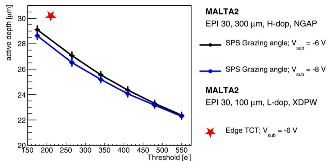
Fig. 12. Active depth versus threshold in electrons for two measurement techniques: grazing angle, performed with a 180 \text{ GeV} hadron beam at SPS CERN and E-TCT, performed with a pulsed laser.
