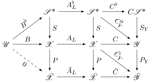
Fig. 6. Commutative diagram for WOR systems. In the diagram, \tilde{\mathcal{X}} := \mathcal{X}/\mathcal{S}^* and \tilde{\mathcal{Y}} := \mathcal{Y}/(C\mathcal{S}^*) . S : \mathcal{S}^* \rightarrow \mathcal{X} is the insertion map of \mathcal{S}^* in \mathcal{X} , S_Y : C\mathcal{S}^* \rightarrow \mathcal{Y} is the insertion map of C\mathcal{S}^* in \mathcal{Y} , P : \mathcal{X} \rightarrow \tilde{\mathcal{X}} is the canonical projection modulo \mathcal{S}^* , and P_Y : \mathcal{Y} \rightarrow \tilde{\mathcal{Y}} is the canonical projection modulo C\mathcal{S}^* . The codomain restriction B^b : \mathcal{U} \rightarrow \mathcal{S}^* is well-defined since \text{Im } B \subseteq \mathcal{S}^* , and the map \bar{C} : \tilde{\mathcal{X}} \rightarrow \tilde{\mathcal{Y}} is well-defined due to the fact that \text{Ker } \bar{C}_Y = \text{Ker } P_Y C = \mathcal{S}^* + \text{Ker } C \supseteq \mathcal{S}^* . The map A_L^b : \mathcal{S}^* \rightarrow \mathcal{S}^* is the restriction of A_L to the A_L -invariant subspace \mathcal{S}^* . The map \bar{A}_L : \tilde{\mathcal{X}} \rightarrow \tilde{\mathcal{X}} is the map induced on \tilde{\mathcal{X}} by A_L .
