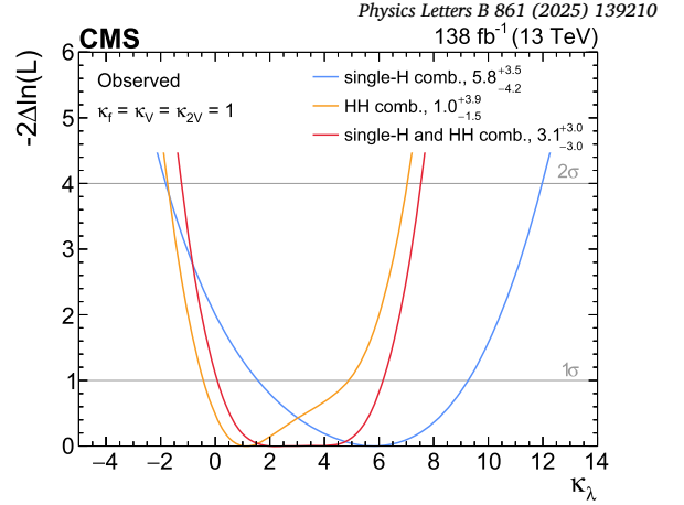
Fig. 4. Observed profile likelihood scans of \kappa_\lambda comparing the full combination of single-H and HH (red) to the combinations of only single-H (blue) or only HH (yellow) channels. The legend includes the best-fit values and the 1\sigma uncertainties.
