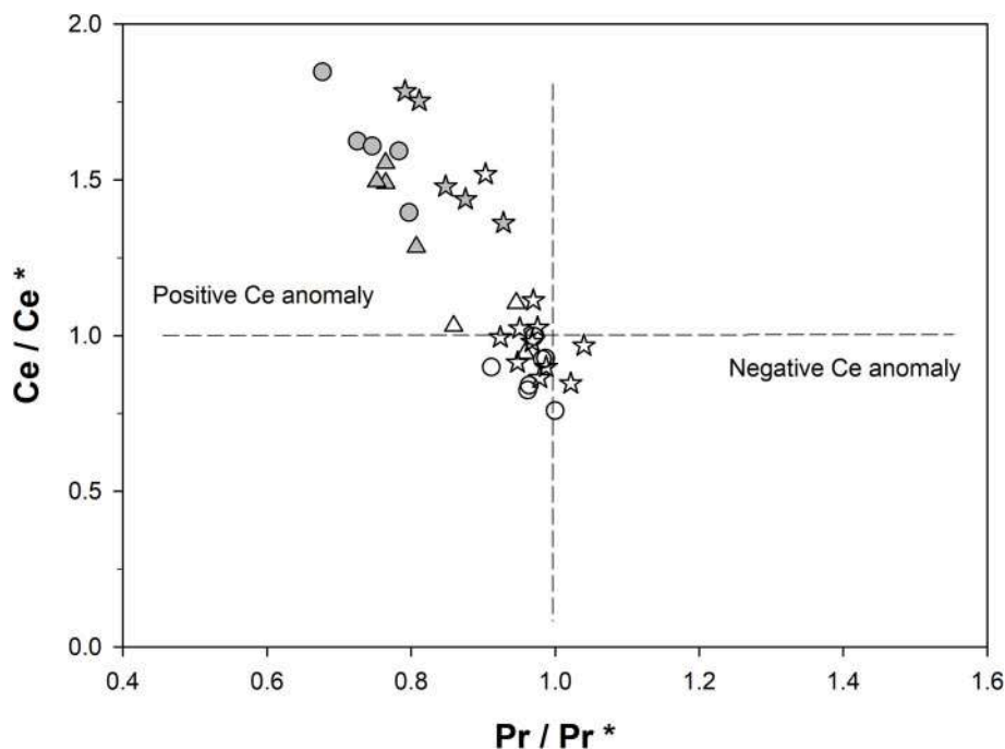
Fig. 12. Location of the studied samples in the McLennan (2001) normalized plots of (\text{Ce}/\text{Ce}^*) vs (\text{Pr}/\text{Pr}^*) labelled as (\text{Ce}/\text{Ce}^*)_N and (\text{Pr}/\text{Pr}^*)_N , respectively. Adapted from Kowal-Linka et al. (2014). Symbols like in Fig. 8.
