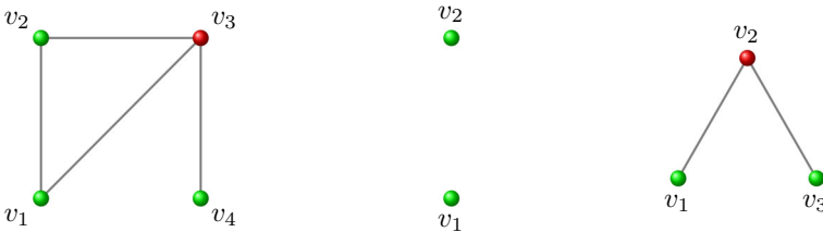
Fig. 2 Some tolerance relations discussed in the text
