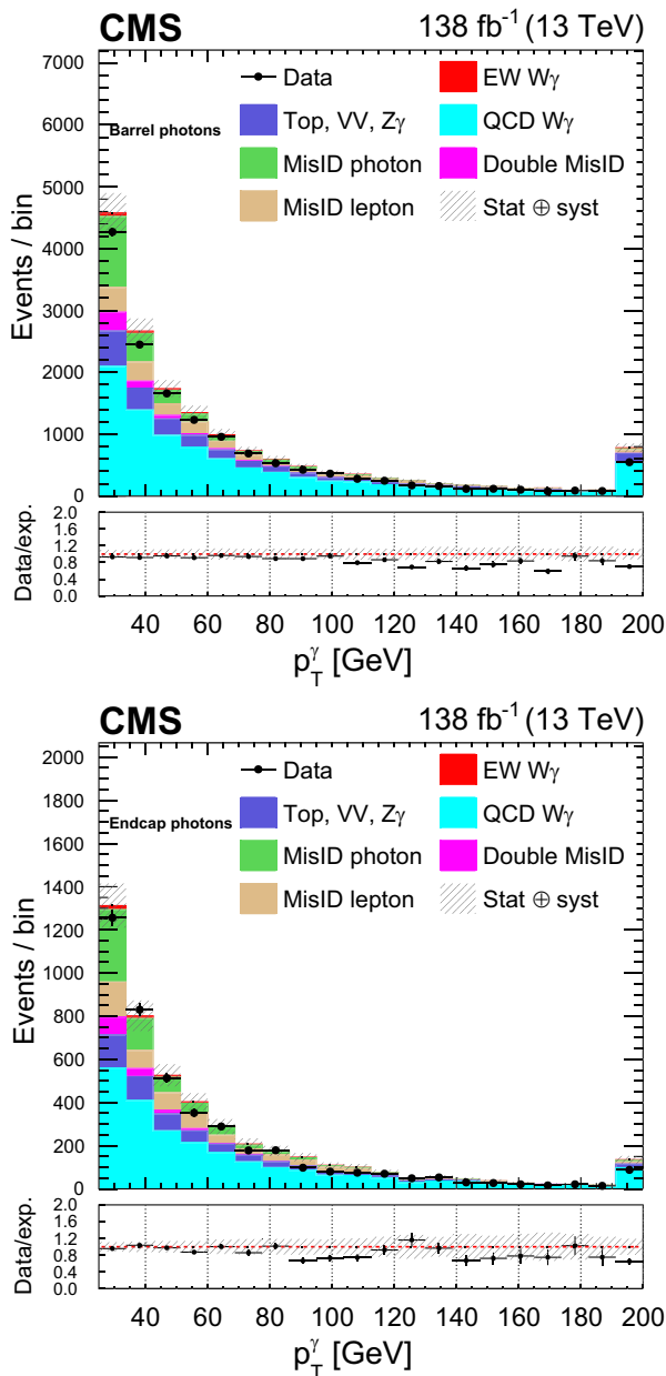
FIG. 2. p_T distributions for photons in the barrel (upper) and in the end caps (lower) in the control region for data and from background estimations before the fit to the data. The misID backgrounds are derived from data, whereas the remaining backgrounds are estimated from simulation. All events with a photon p_T > 200 GeV are included in the last bin. The hatched bands represent the combined statistical and systematic uncertainties on the predicted yields. The vertical bars on the data points represent the statistical uncertainties of data. The bottom panels show the ratios of the data to the predicted yields.
