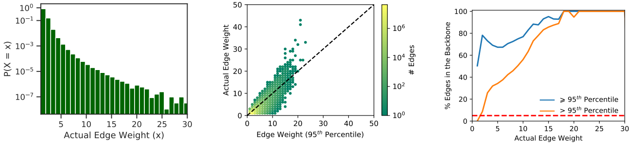
(a) Probability distribution of edge weights \gamma(cd) in the original graph G_P . (b) Actual edge weight \gamma(cd) compared with null model edge weight \hat{\gamma}_{95}(cd) . (c) Fraction of edges included in the backbone B_P , separately for different values of \gamma .
