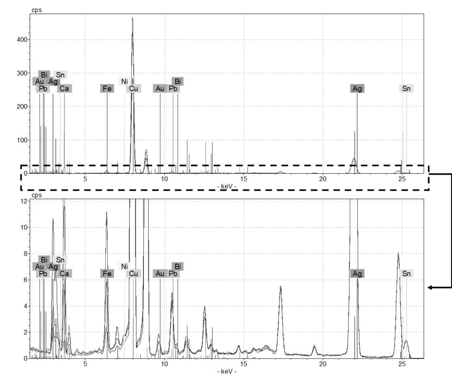
Figure 1. Four overlapped \mu -EDXRF spectra of the coin no. D27. Spectrum of recto_1 in pink, recto_2 in blue, verso_1 in red, and verso_2 in green. The lower spectrum is relative to the area within the dashed frame, so that even the lower intensity peaks can be appreciated.
