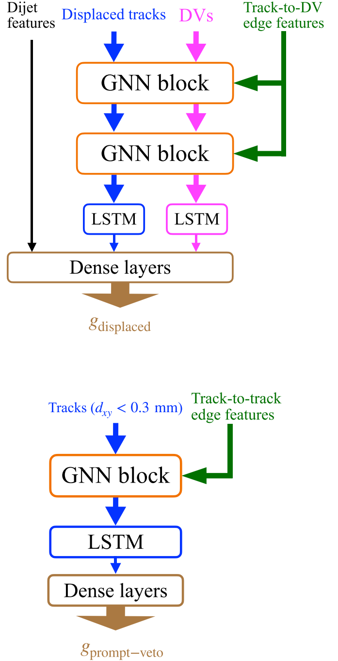
Figure 2. The architectures of the displaced (upper) and prompt-veto (lower) taggers. The displaced tagger takes as input the dijet global features, displaced tracks, and DVs. The prompt-veto tagger takes as input the tracks with d_{xy} < 0.3 mm.
