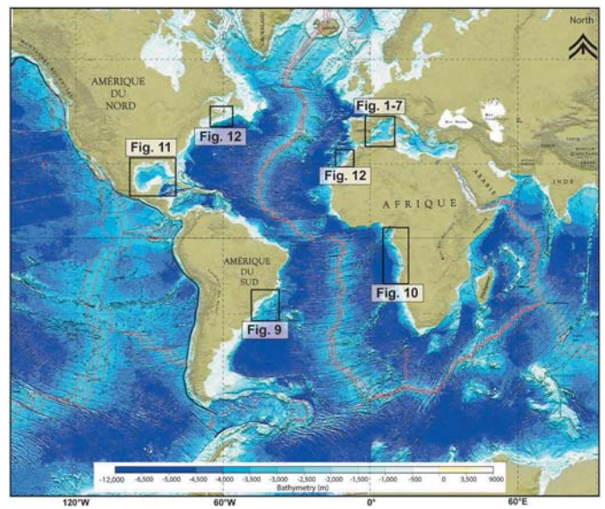
Fig. 8. Regional bathymetric map showing location of the world passive margins study areas.
