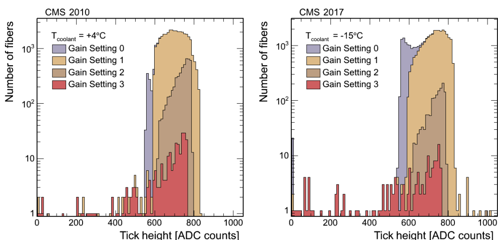
Figure 11. Example distributions of tick heights for each of the four laser driver gain settings for data taken in 2010 at +4°C coolant temperature (left) and in 2017 at -15°C coolant temperature (right). Distributions from different gain settings are stacked.
