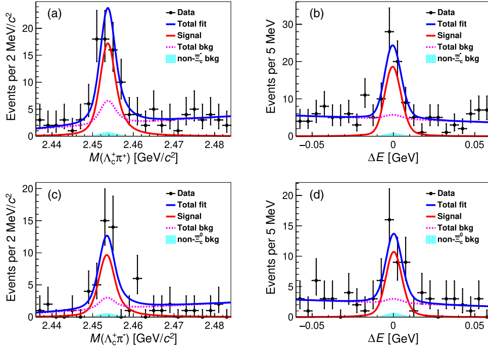
FIG. 2. Distributions of (a, c) M(\Lambda_c^+\pi^\pm) and (b, d) \Delta E for the reconstructed (top) B^+ \rightarrow \Sigma_c(2455)^{++}\bar{\Xi}_c^- and (bottom) B^0 \rightarrow \Sigma_c(2455)^0\bar{\Xi}_c^0 candidates, using events from the signal regions of M(\bar{\Xi}_c^{-,0}) in the combined Belle and Belle II datasets. Points with error bars are the data, the solid blue curves show the total fit results, the solid red curves correspond to the fitted signal components, and the dashed magenta curves represent the total fitted background components. The shaded cyan regions show the peaking-background contributions from the inclusive B^{+,0} \rightarrow \Sigma_c(2455)^{+,0}X decays, where X \neq \bar{\Xi}_c^{-,0} .
